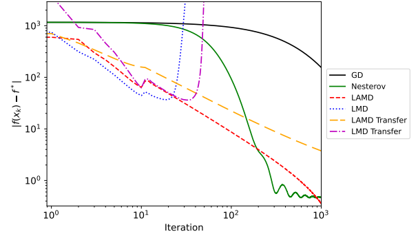
Fig. 4: Plot of f(x^{(k)}) - f^* for LMD and LAMD for de-noising with swapped mirror maps. Adding momentum and using the mirror map of LMD (yellow) gives long-term stability. Training with LAMD also adds stability to the mirror maps when applied without momentum (purple).
