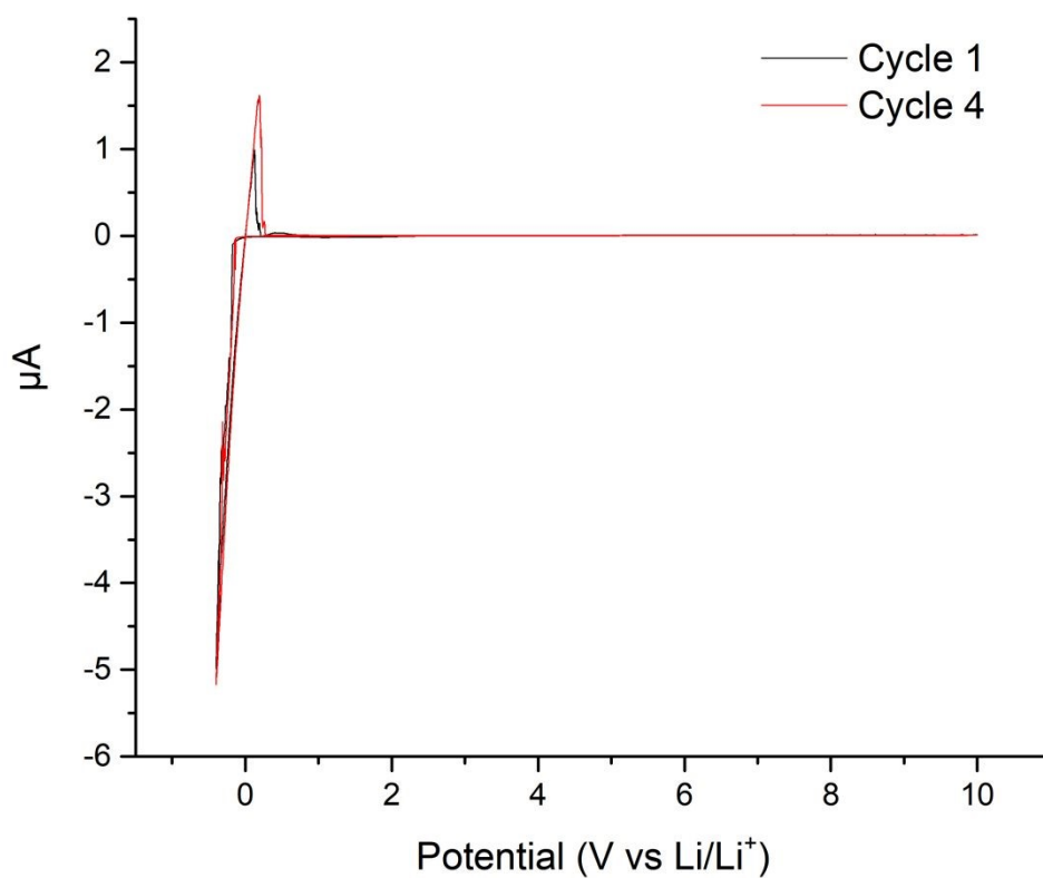
Figure 6. Cyclic voltammetry of LTC at room temperature using an Au/LTC/Li cell.
