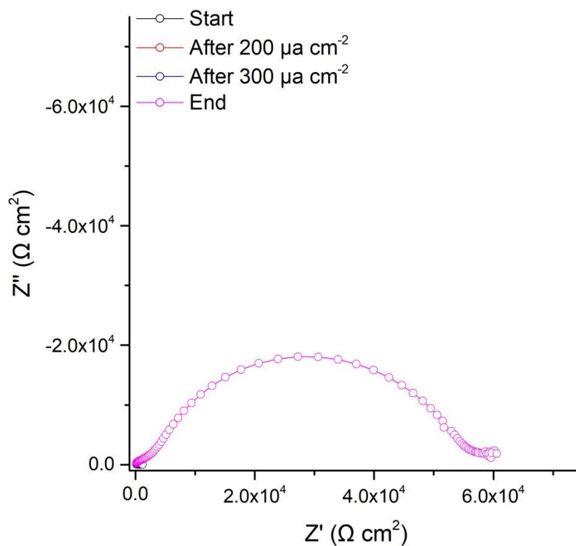
Figure 7. Symmetry cell impedance spectra and CCD measurements where a) is the CCD data measured in increments of 10 \mu\text{A cm}^{-2} , stars indicate where cell was stopped for impedance analysis. b) is the overlaid impedance spectrums during the CCD testing at different current densities at room temperature and c) the same as figure 7b but with final impedance spectrum showing interfacial degradation upon cell failure (additional long term cycling, at differing current densities, is available in figure S8.)
