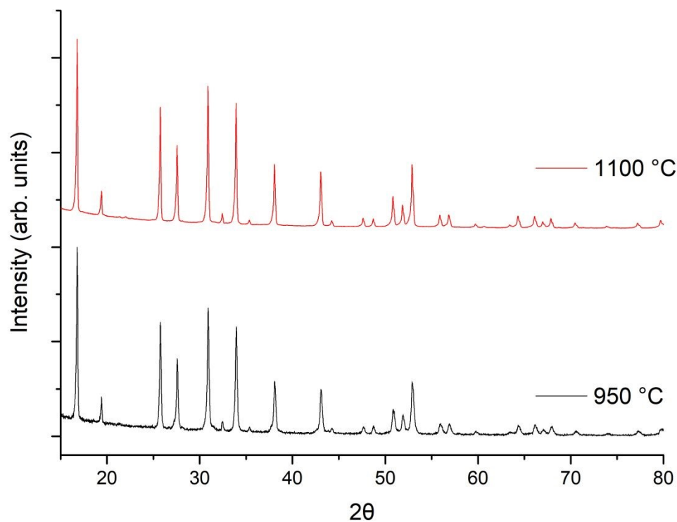
Figure 1. XRD patterns of LTC sintered in powder form (950°C, 100°C min -1 ) and as a pellet (1100°C, 40°C min -1 ). Both samples were sintered for 1h and demonstrate pure garnet ( 1a\bar{3}d ) type symmetry. In both cases heating rates were the maximum available for the furnace model.
