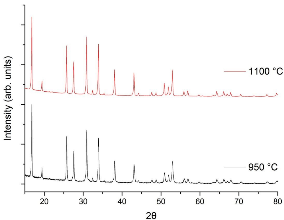
Figure 1. XRD patterns of LTC sintered in powder form (950°C, 100°C min -1 ) and as a pellet (1100°C, 40°C min -1 ). Both samples were sintered for 1h and demonstrate pure garnet ( Ia\bar{3}d ) type symmetry. In both cases heating rates were the maximum available for the furnace model.
