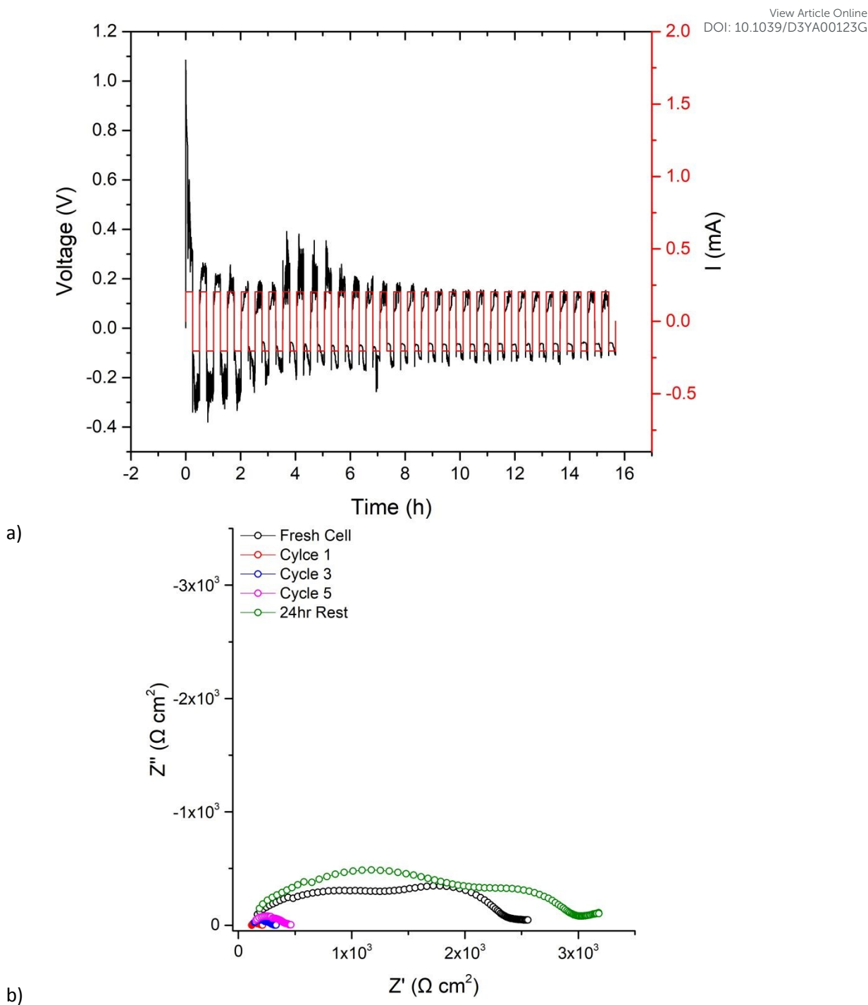
Figure 9. After the first cycle at 500 \mu\text{A cm}^{-2} and the corresponding impedance analysis in figure 8 was complete, LTC cycling was restarted at 500 \mu\text{A cm}^{-2} and results are shown for a) 31 cycles with the corresponding impedance analysis in b) taken as per figure 8b.
