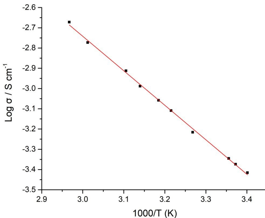
Figure 5. Arrhenius plot of LTC over the temperature range of 19 – 64 °C (activation energy = 0.34 eV).
