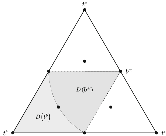
Fig. 5 Strictly concave power:
