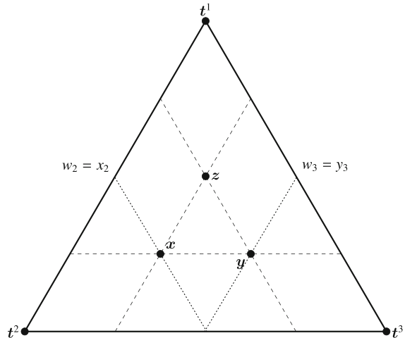
Fig. 2 Triangular, internally stable \mathbf{x} , \mathbf{y} and \mathbf{z} with x_1 = y_1 , y_2 = z_2 and z_3 = x_3
