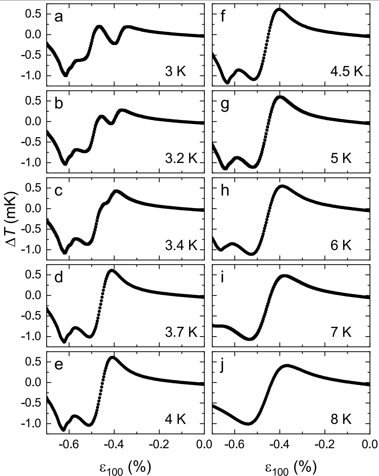
Extended Data Fig. 2 | Response of the elastocaloric effect as a function of strain (further data: high temperatures). \Delta T(\epsilon_{100}) recorded at 1,513 Hz with an excitation amplitude \epsilon_{100}^{\text{exc}} between 2.9 \times 10^{-6} and 3.5 \times 10^{-6} during strain sweeps at ten different temperatures from 3 K to 8 K.
