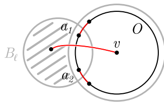
FIGURE 7. In the depicted situation, the separator of the pseudo-reduction induced by \ell consists of the red edges
