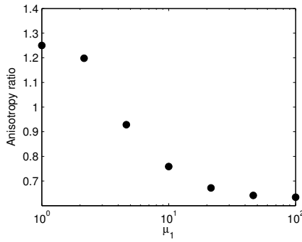
Fig. 10: The anisotropy ratio of the resulting distribution of cells as \mu_1 is varied.
