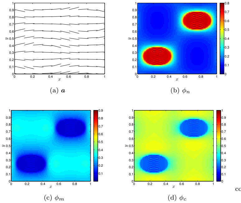
Fig. 11: Simulation results at time t = 4.7 with high extensional viscosity in the fibre direction ( \mu_2 = 10 ): (a) fibre alignment, \mathbf{a} ; (b) cell volume fraction, \phi_n ; (c) medium volume fraction, \phi_m ; (d) collagen volume fraction, \phi_c . All other parameters and initial conditions as in Table 1.
