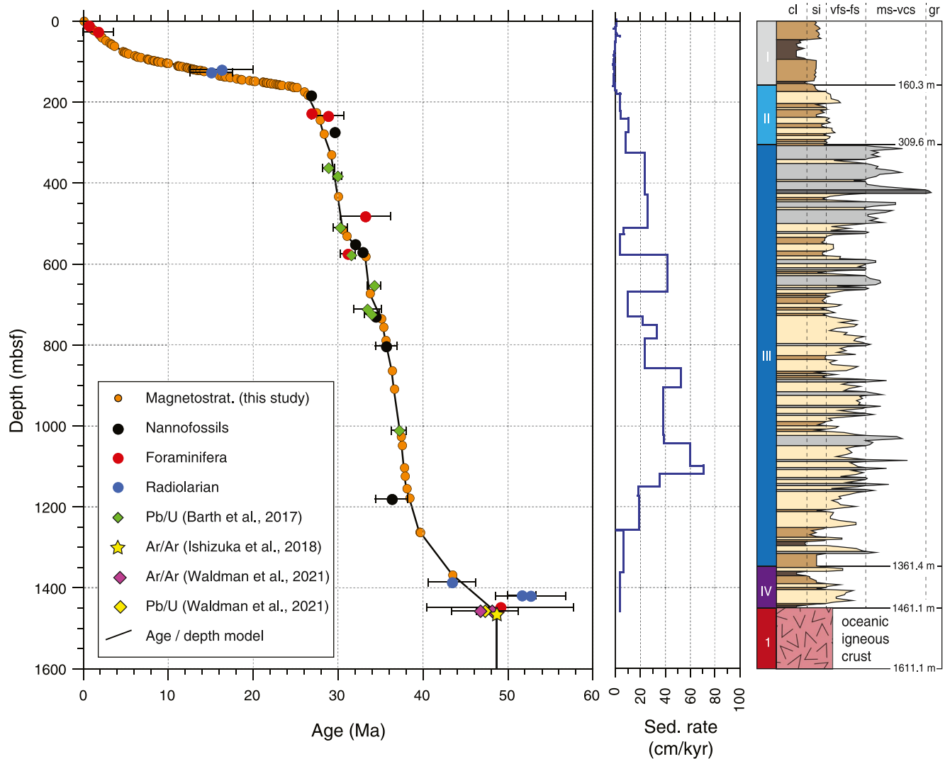
Figure 4. (Left) Age/depth model obtained from the magnetostratigraphic ages; (center) sedimentation rates calculated after decompaction (see text); (right) Lithostratigraphic log of Site U1438 after Arculus et al. (2015b).
