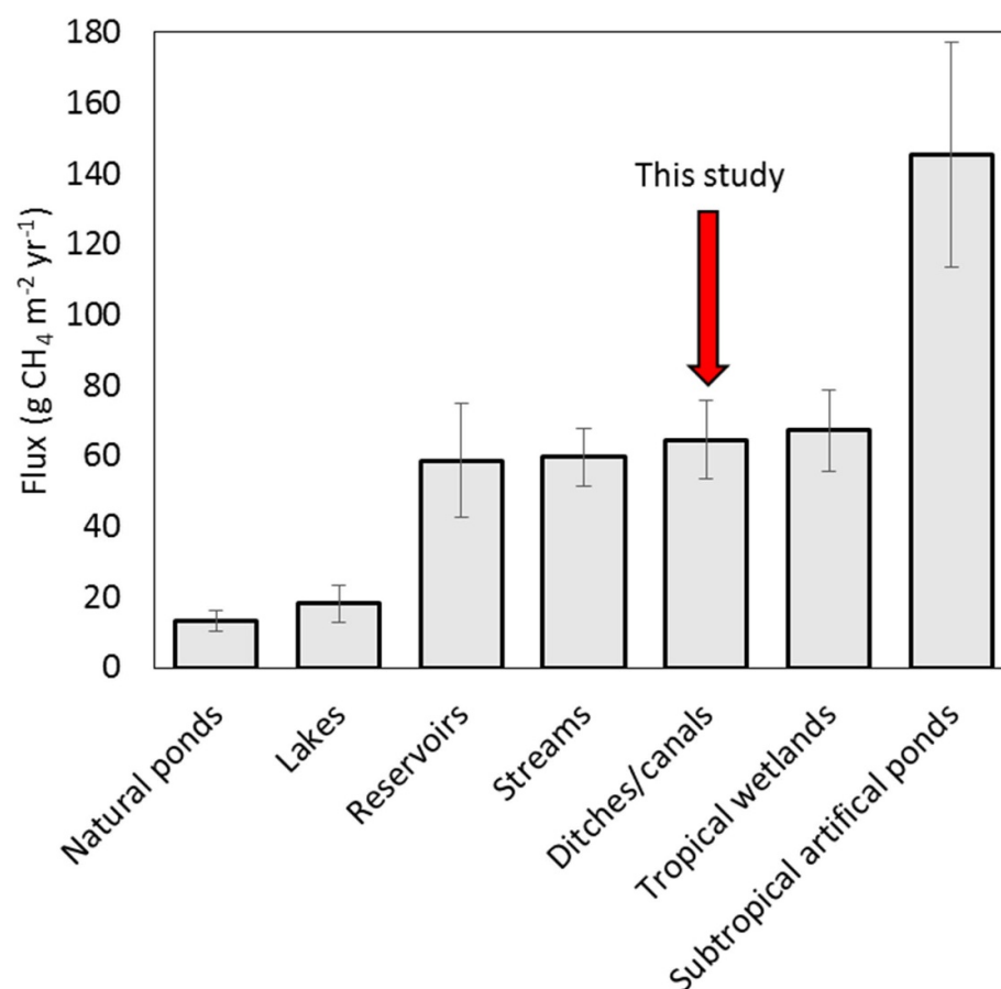
Figure 3. Comparison of mean annual fluxes from different freshwater systems. Data: natural ponds ( n = 50 ) 8 , lakes ( n = 96 ) 10 , reservoirs ( n = 75 ) 4 , streams ( n = 411 ) 13 , ditches/canals ( n = 64 ) tropical wetlands ( n = 54 ) [63] and subtropical artificial ponds ( n = 33 ) 9,14 . Error bars show standard error of the mean. See SI text 6 for further detail.
