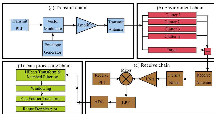
FIGURE 1 Schematic of the front end model of the monostatic radar in simulation. The front end consists of four main sections. The transmit chain transmits the pulsed sinusoidal signal to the environment through the transmit antenna. The clutter and targets in the environment reflect the signal to the radar receive antenna. In the receive chain, the received signal undergoes stages of amplification and down-conversion to generate an intermediate frequency signal. The intermediate frequency signal gets converted to a baseband signal in the data processing chain. The baseband signal undergoes further data processing stages to enhance the target's signal-to-noise ratio. The building blocks in the transmit chain, the environment chain, and the receive chain are modelled as separate blocks in Simulink. The building blocks in the data processing chain were generated using a separate code written in MATLAB.
