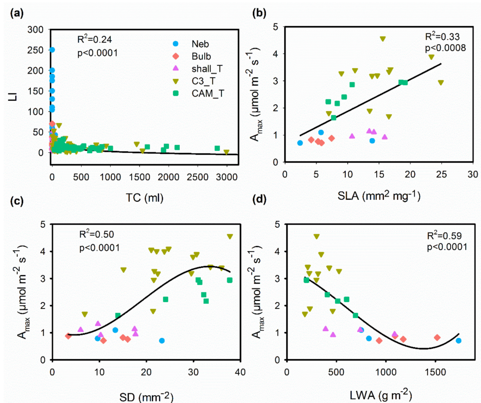
Figure 5. Significant relationships of functional trait across the five functional groups of epiphytic Bromeliaceae; (a) leaf index (LI) versus tank capacity (TC); (b) light saturated photosynthetic rate per leaf area ( A_{\max} ) versus specific leaf area (SLA); (c) A_{\max} versus stomatal density (SD); (d) A_{\max} versus leaf water content on area basis (LWA). Each point corresponds to the mean value per species. Point colors correspond to the following functional groups: Bulb = pseudobulbs (pink); C3_T = C 3 tanks (yellow); Shall_T = shallow tanks (purple); CAM_T = CAM tanks (green); Neb = nebulophytes (blue).
