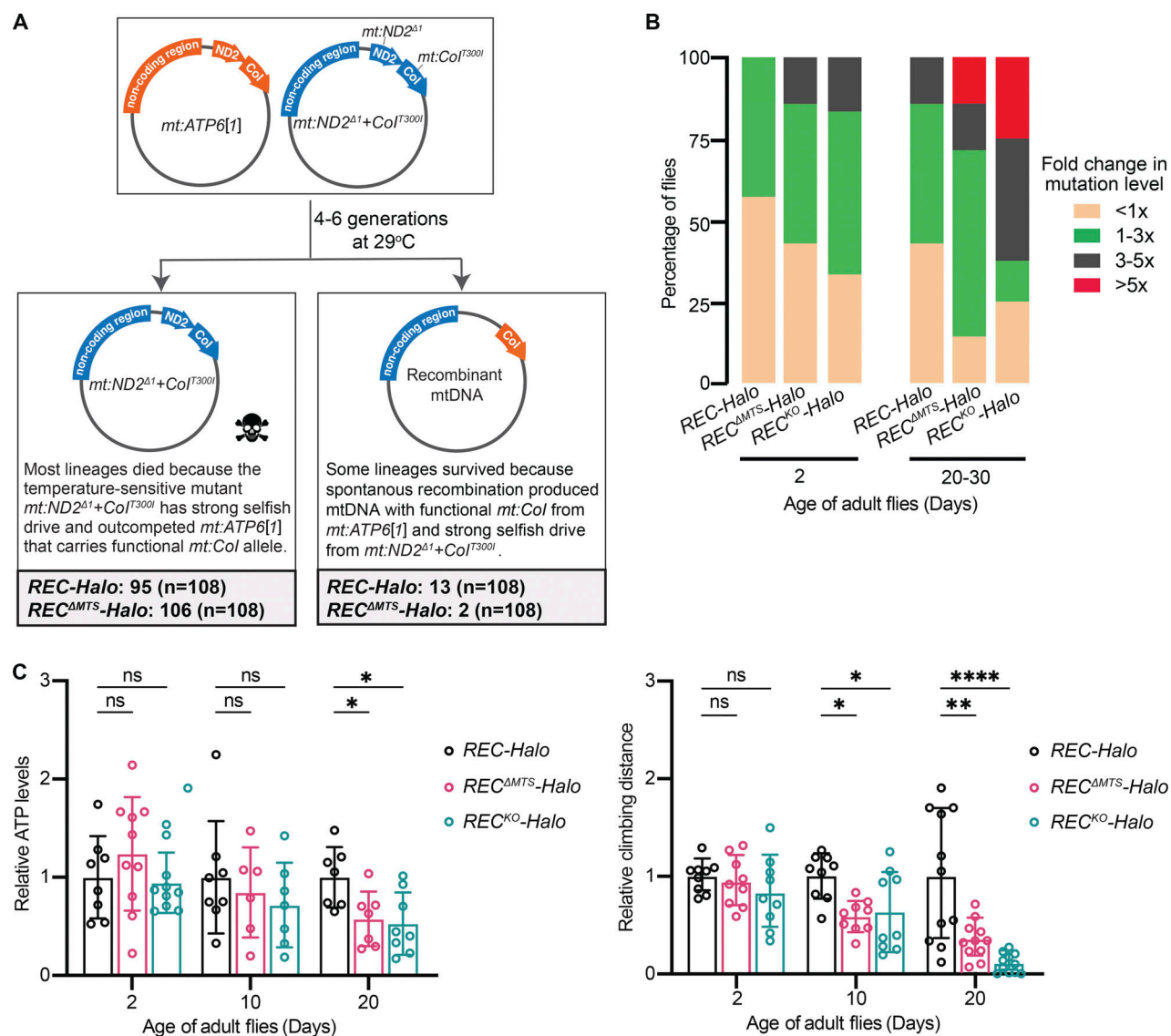
Figure 4. REC mediates spontaneous recombination and safeguards mtDNA during ageing. (A) Numbers of recombinant mitochondrial genomes generated in REC-Halo and REC ΔMTS -Halo flies heteroplasmic for mt:ATP6[1] and mt:ND2 Δ1 +Col T300I from 108 lineages. (B) Stacked bar plots showing the percentage of flies with different levels of mtDNA mutations. The number of mtDNA variants (above 1% heteroplasmy) detected in individual flies was divided by the average number of mtDNA variants detected in 2-d-old REC-Halo fly population to calculate the fold change in mtDNA mutation levels ( n = 6-8 flies for each genotype of a given age). (C) Relative ATP levels and climbing distance in young and aged flies (ATP levels: n = 6-10 groups of 5 males; average distance climbed: n = 9-14 groups of 8 males). Data represent mean \pm SD, two-way ANOVA with Dunnett's multiple comparisons, ns P > 0.05 , * P < 0.05 , ** P < 0.01 , **** P < 0.0001 .
