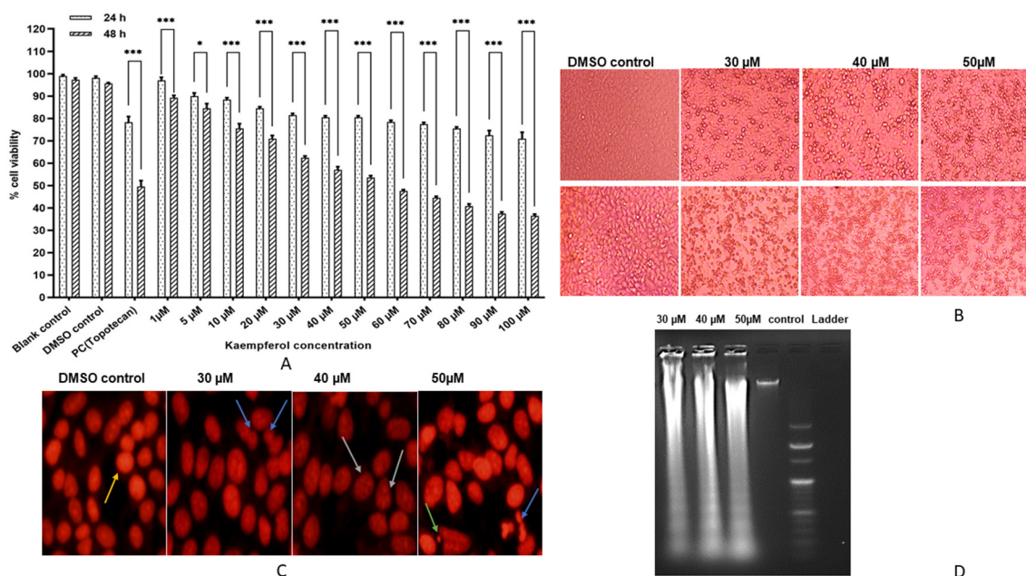
Figure 1. Kaempferol exhibits cytotoxic effect on HeLa cells (A) Graph presenting concentration and time dependent reduction in cell viability of HeLa cells after treatment with kaempferol (1–100 μM)
