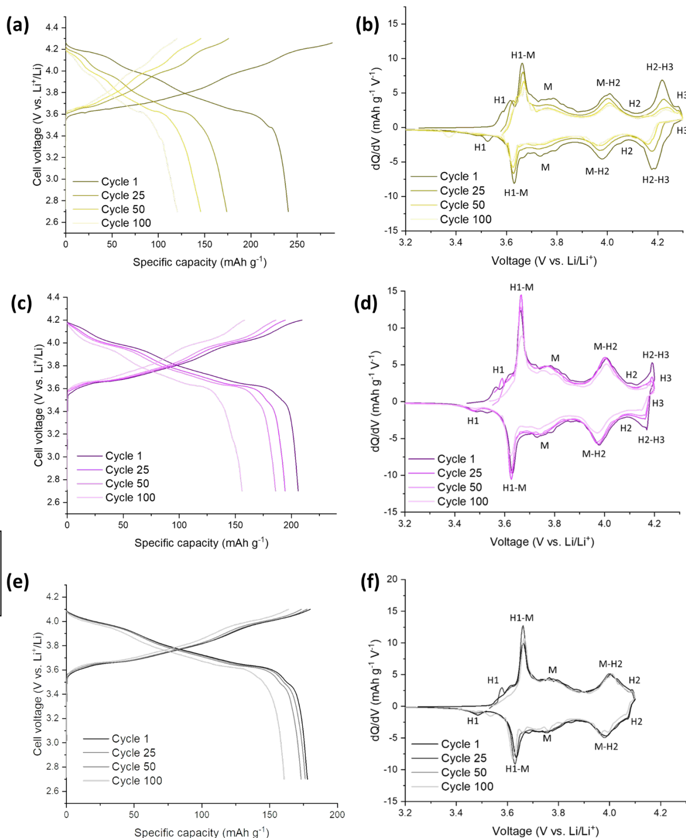
Figure 6- Electrochemical performance during galvanostatic charge and discharge of Mo-LNO/ Li half cells at 10 mA g -1 : (a) between 2.7 - 4.3 V (b) corresponding differential capacity (dQ/dV) plot with phases (c) between 2.7 - 4.2 V (d) corresponding differential capacity (dQ/dV) plot with phases (e) between 2.7 - 4.1 V (f) corresponding differential capacity (dQ/dV) plot with phases.
