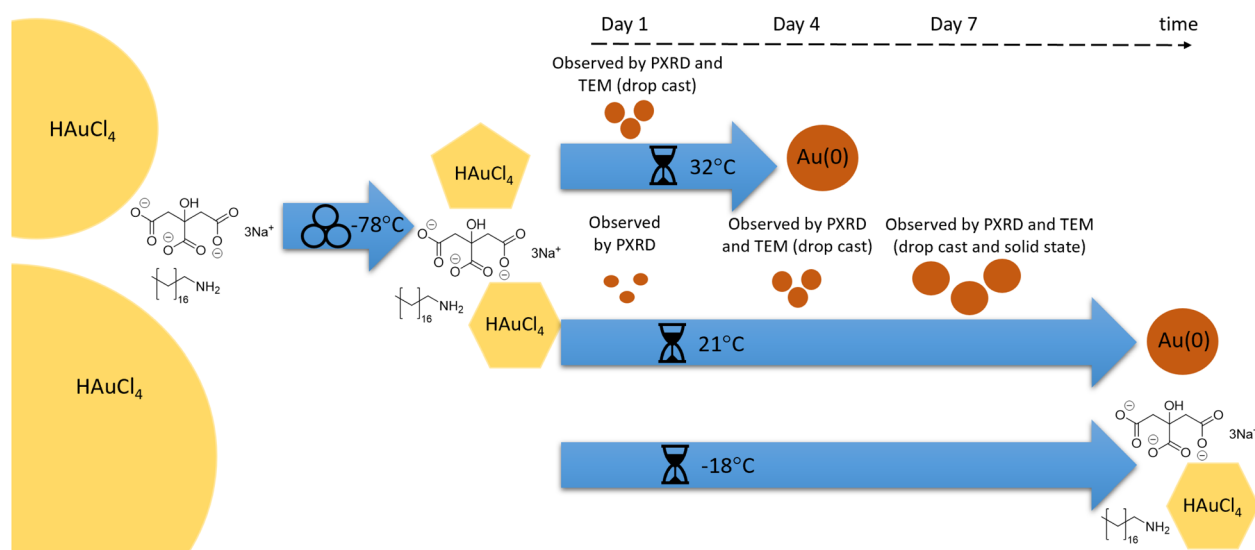
Fig. 7 Schematic representation of the synthetic sequence: precursors HAuCl 4 , NaCl and ODA were milled at -78 °C, leading to HAuCl 4 comminution. Aging at -18 °C (LT) led to no reaction; aging at 21 °C (RT) led to gradual reduction and nanoparticle growth, as observed by different techniques; aging at 32 °C (ET) led to a similar outcome in an accelerated sequence.
