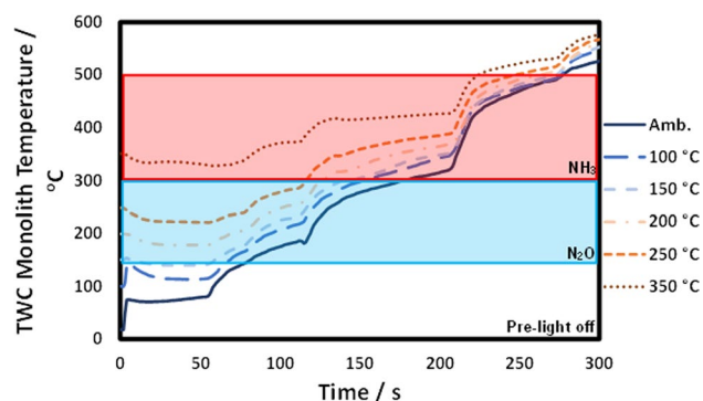
Fig. 8 TWC monolith inlet face temperature for each catalyst starting temperature. Note the highlighted temperature regions for \text{NH}_3 and \text{N}_2\text{O} formation
