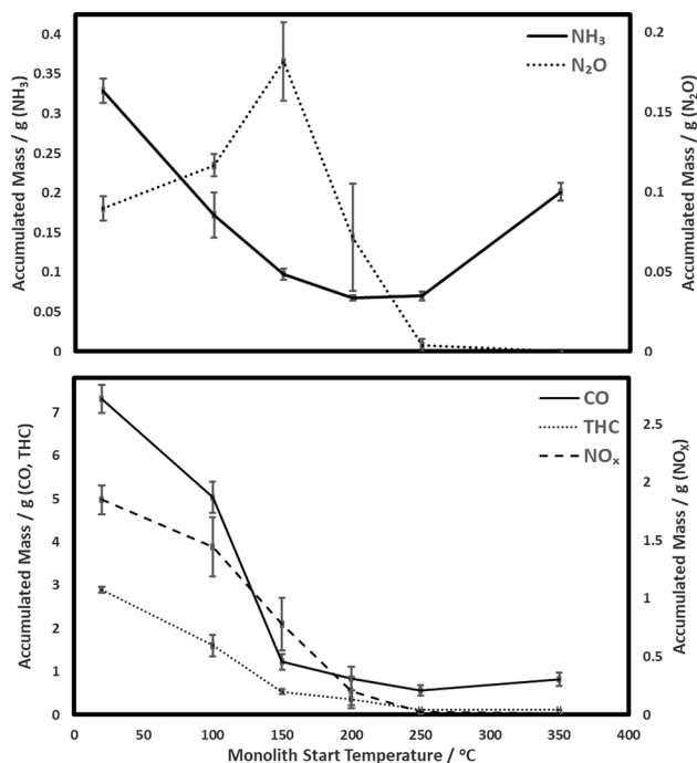
Fig. 9 Accumulated mass of emissions for the first 500 s of engine operation with respect to the TWC temperature at the time of engine start for \text{NH}_3 , \text{N}_2\text{O} , \text{CO} , \text{NO}_x and \text{THC} . Confidence intervals show the 95% confidence level calculated from 3 repeats of the start-up test
