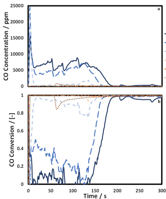
Fig. 4 a Post-TWC CO concentration and b TWC CO conversion efficiency
