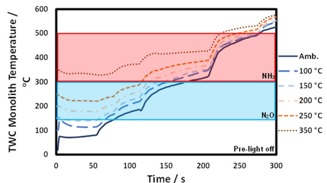
Fig. 8 TWC monolith inlet face temperature for each catalyst starting temperature. Note the highlighted temperature regions for NH 3 and N 2 O formation
