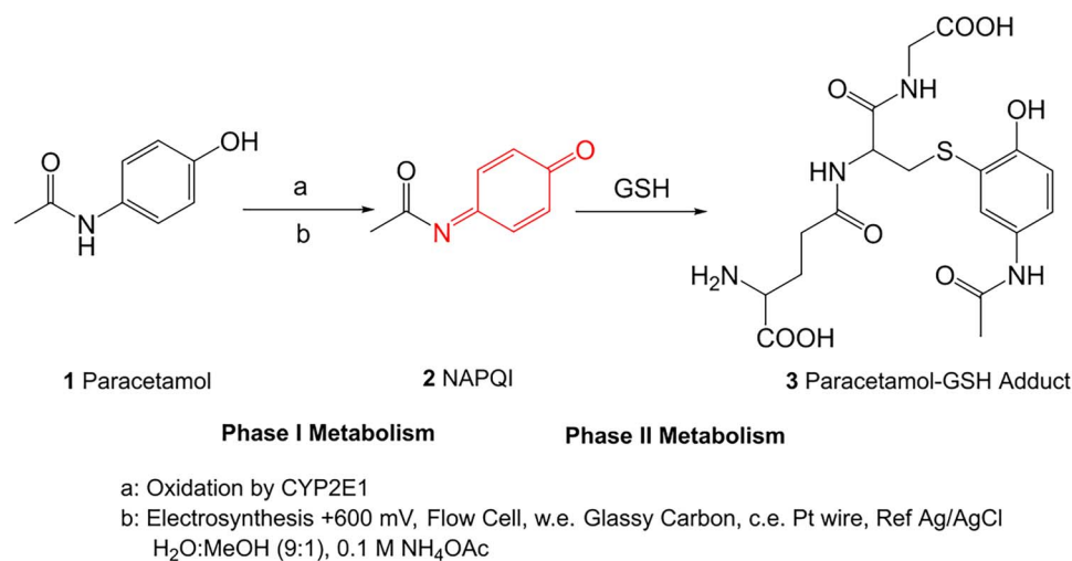
Fig. 2. Electrochemical phase I and II metabolic mimicry of paracetamol oxidation and GSH adduct formation.
