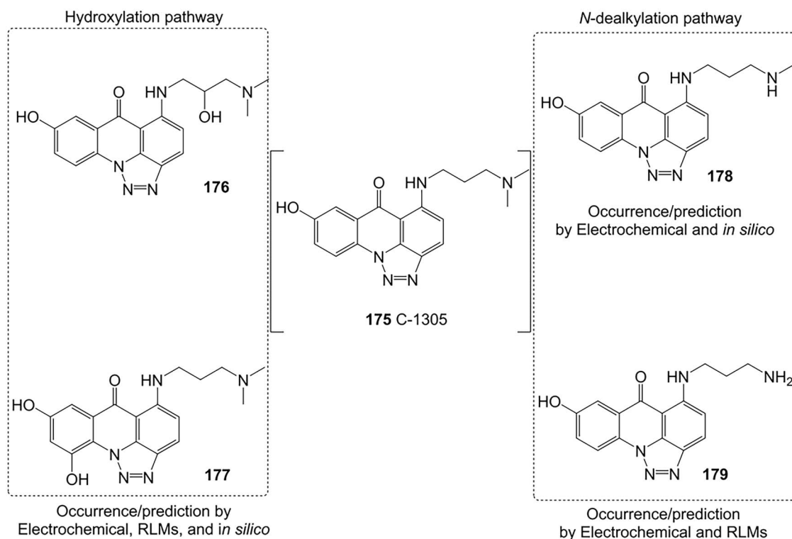
Fig. 14. Phase I metabolism simulation of 5-dimethylaminopropylamino-8-hydroxytriazoacridinone (C-1305). ES conditions: WE: GC, flow rate 20 μL/min, potential 0–2500 mV (10 mV steps), electrolyte: 0.1% HCO 2 H in water/CH 3 OH (50:50, v/v).
