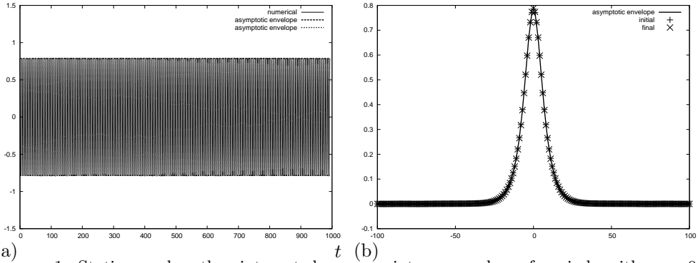
FIGURE 1. Stationary breather integrated over an integer number of periods with \epsilon = 0.1 : (a) \hat{u}_0(t) and its asymptotic envelope u_{max}(0, t) for 0 \leq t \leq t_{end} and (b) \hat{u}_n(0) , \hat{u}_n(t_{end}) and u_{max}(x, t_{end}) .
