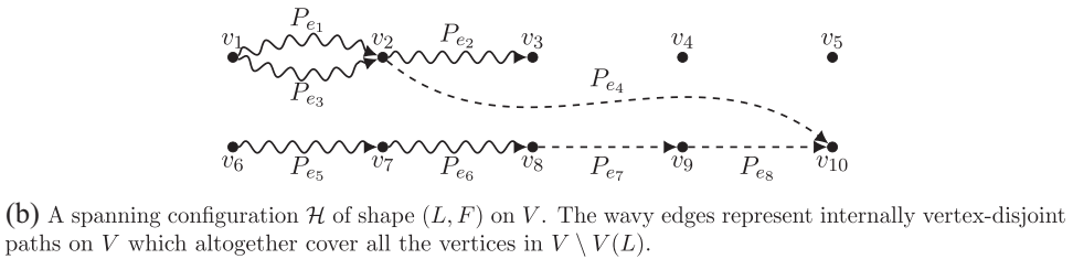
FIGURE 2 A layout (L, F) and a spanning configuration of shape (L, F) . Dashed edges represent fixed edges (that is, the edges of F ).
