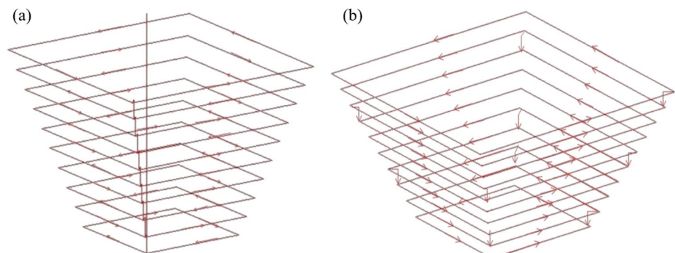
Fig. 18 Tool path design. a Contour (z-level) profile, b helical (spiral) profile [68]
