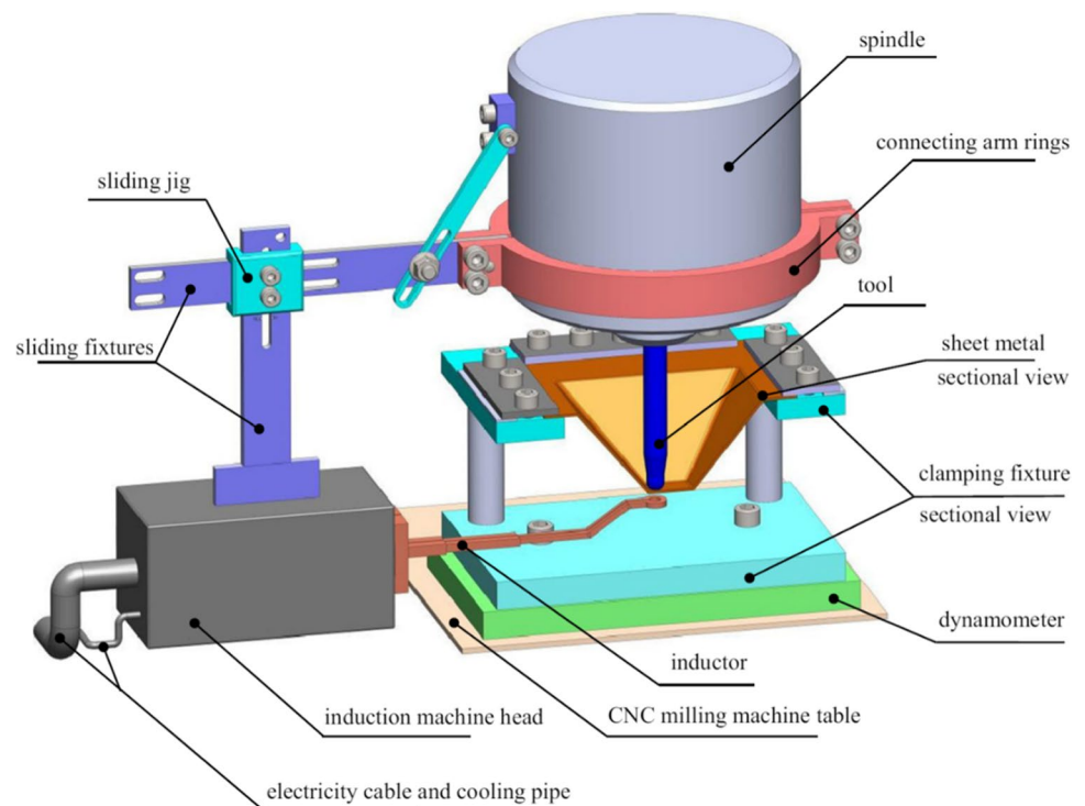
Fig. 8 Illustration of induction heating-assisted SPIF system [16]
