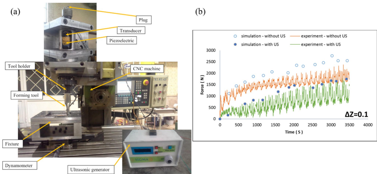
Fig. 2 Experimental setup of UVSPIF process. a Illustration of UVSPIF, b measured forming force from the UVSPIF process. US, ultrasonic forming force [39]
