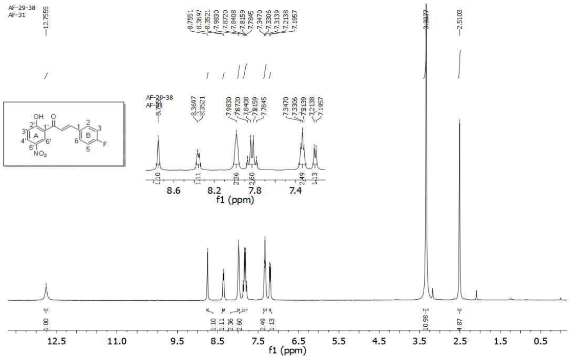
Figure S1: 1 H NMR of 3a
