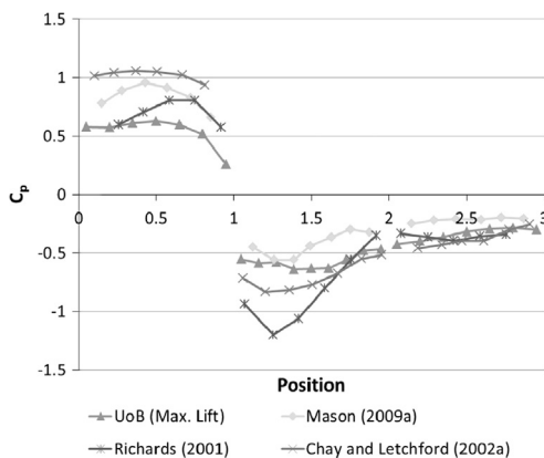
Fig. 13. Centreline pressure coefficients over a cube at 0° yaw during simulated thunderstorm downbursts and full-scale ABL flow. Position is normalised by the cube size.
