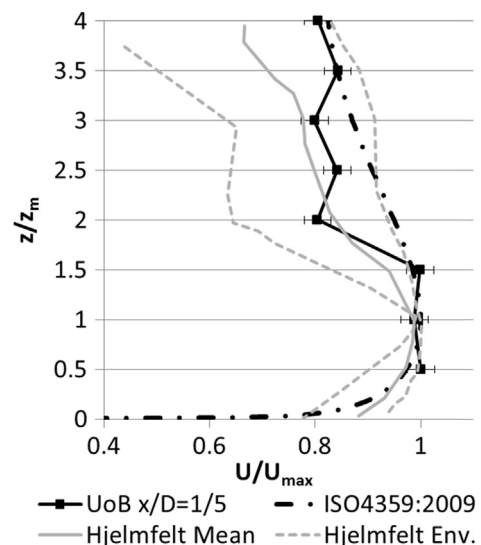
Fig. 7. Vertical velocity profiles – UoB, full-scale (mean and upper and lower envelopes from Hjelmfelt (1988)) and the ISO4359 thunderstorm profile.
