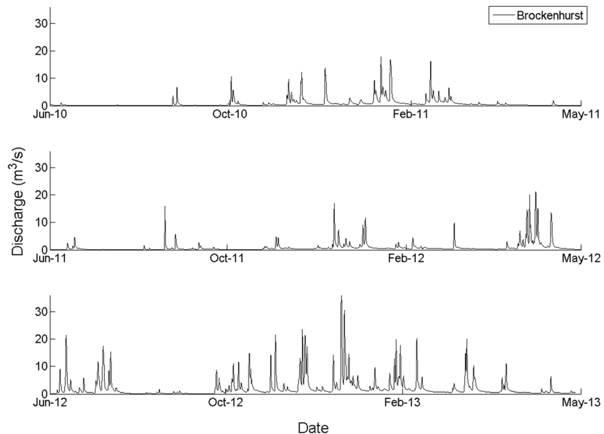
Figure 2. Hydrograph of flows at Lymington River at Brockenhurst gauging station for the duration of the study.
