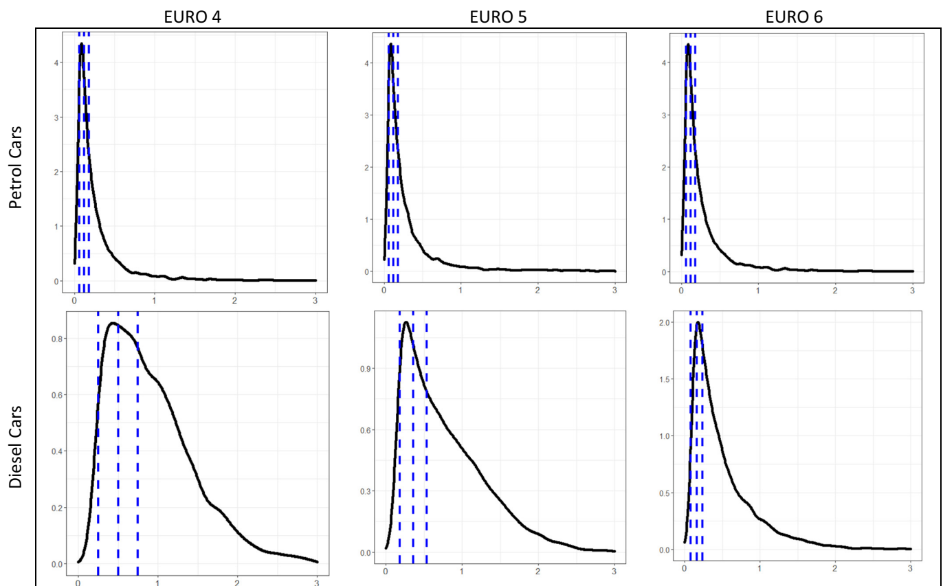
Fig. 2. The probability distribution function of the real-world NO x emission factors measured by EDAR for petrol and diesel passenger cars. The blue dashed lines represent 1 ×, 2 × and 3 × the type-approved emission limits for the given EURO class and fuel type. The y and x-axis labels are density and emission factor, (g/km), respectively.
