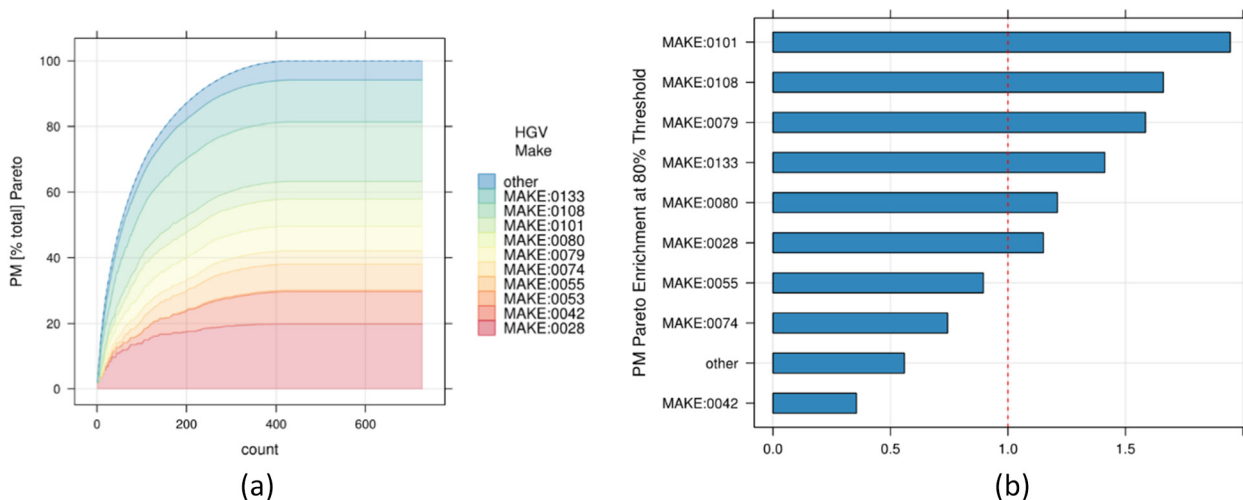
Fig. 8. (a) Pareto plot, and (b) Pareto enrichment plot for different makes of HGV PM emissions.
