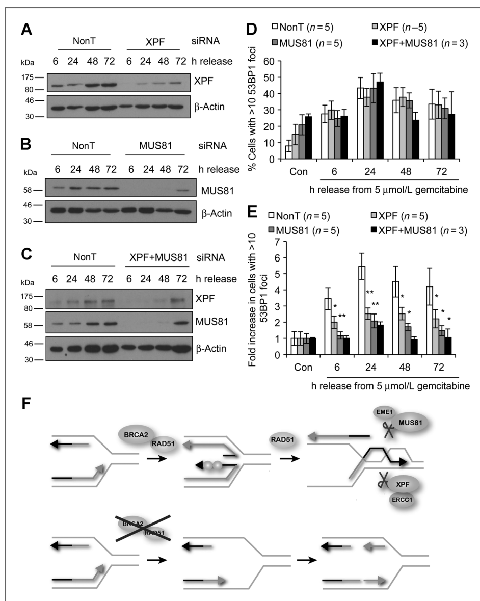
Figure 6. Gemcitabine-induced DSBs depend on MUS81 and XPF. A , protein levels of XPF and \beta -actin (loading control) after transfection with nonT or XPF siRNAs for 72 hours, treated with 5 \mu M/L gemcitabine for 2 hours and release for the times indicated. B , protein levels of MUS81 after transfection with nonT or MUS81 siRNAs as in A . C , protein levels of XPF, MUS81, and \beta -actin (loading control) after transfection with nonT or MUS81 and XPF siRNAs as in A . D , percentage of U2OS cells \pm XPF and MUS81 displaying more than 10 53BP1 foci after release from gemcitabine. E , quantification of increase in cells displaying more than 10 53BP1 foci as in D (asterisks compared with nonT siRNA). F , suggested model for HR-dependent replication fork slowing and DSB formation. Forks affected by gemcitabine treatment are recognized by BRCA2 and RAD51 and remodeled into joint molecule HR intermediates such as D-loops. These intermediates are preferentially cleaved by MUS81 and XPF. Error bars, SEM; *, P < 0.05 ; **, P < 0.01 , Student t test.
