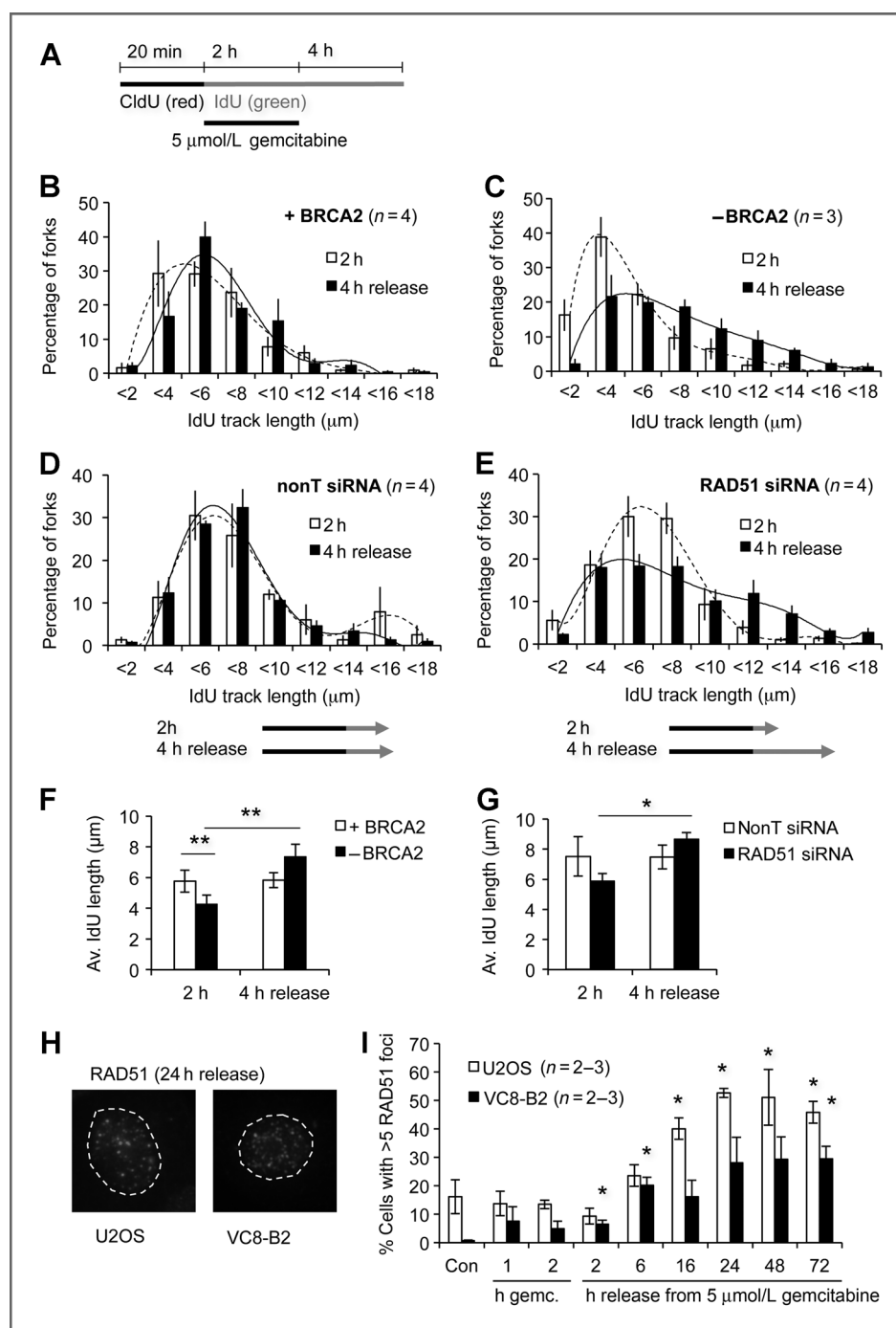
Figure 3. BRCA2 and RAD51 inhibit replication fork progression after release from gemcitabine. A , labeling protocol for DNA fiber analyses. Cells were labeled with CldU, treated with IdU and 5 \mu\text{mol/L} gemcitabine for 2 hours and released into IdU for 4 hours. B , length distributions of IdU-labeled tracks from VC8-B2 cells (+BRCA2). C , length distributions of IdU-labeled tracks from VC8 cells (-BRCA2). D , length distributions of IdU-labeled tracks from U2OS cells treated with nonT siRNA. E , length distributions of IdU-labeled tracks from U2OS cells treated with RAD51 siRNA. F , average lengths of IdU tracks in VC8 and VC8-B2 cells treated as in A . G , average lengths of IdU tracks in U2OS cells \pm RAD51. H , representative images of RAD51 foci in cells released from 5 \mu\text{mol/L} gemcitabine for 24 hours. I , percentages of cells displaying more than 5 RAD51 foci during 1 and 2 hours gemcitabine treatment and after release from gemcitabine (asterisks compared with Con). Error bars, SEM; *, P < 0.05 ; **, P < 0.01 , Student t test.
