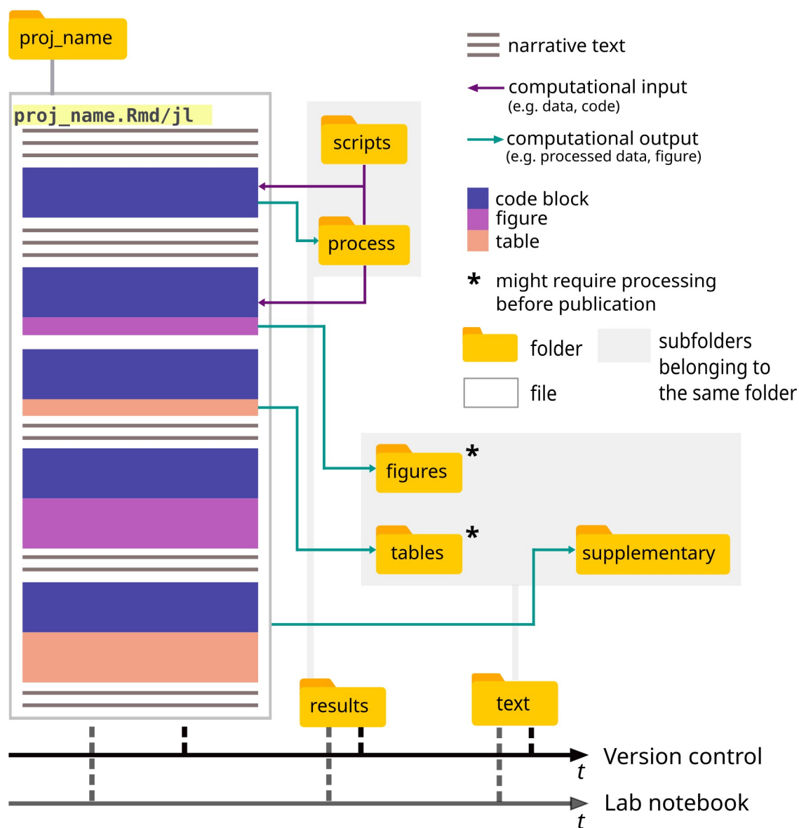
Fig 2. Schematics of the organization of a research project (proj_name) around a computational notebook (proj_name.Rmd/jl, referring to an RMarkdown or Julia file). The notebook contains narrative text supplementary to the manuscript's main text, as well as text explaining the reasoning behind the computational work (included as code blocks) and its respective outputs (either kept on the notebook or saved as figures or tables). The notebook stays at upper level of a file structure (Fig 1), which provides easy access to all relevant folders for input (purple) and output (green) files through relative paths. The gray area shows subfolders that are nested inside folders (e.g., the figures and tables folders are inside the text folder). The notebook, along with all the files in the project's folder, can be subjected to version control and be referenced in a lab notebook, thanks to the nested structure of the project. We recommend publishing it as your main supplementary material to the manuscript, along with a rendered version (.pdf or .html), any scripts, and not yet public data you use.
