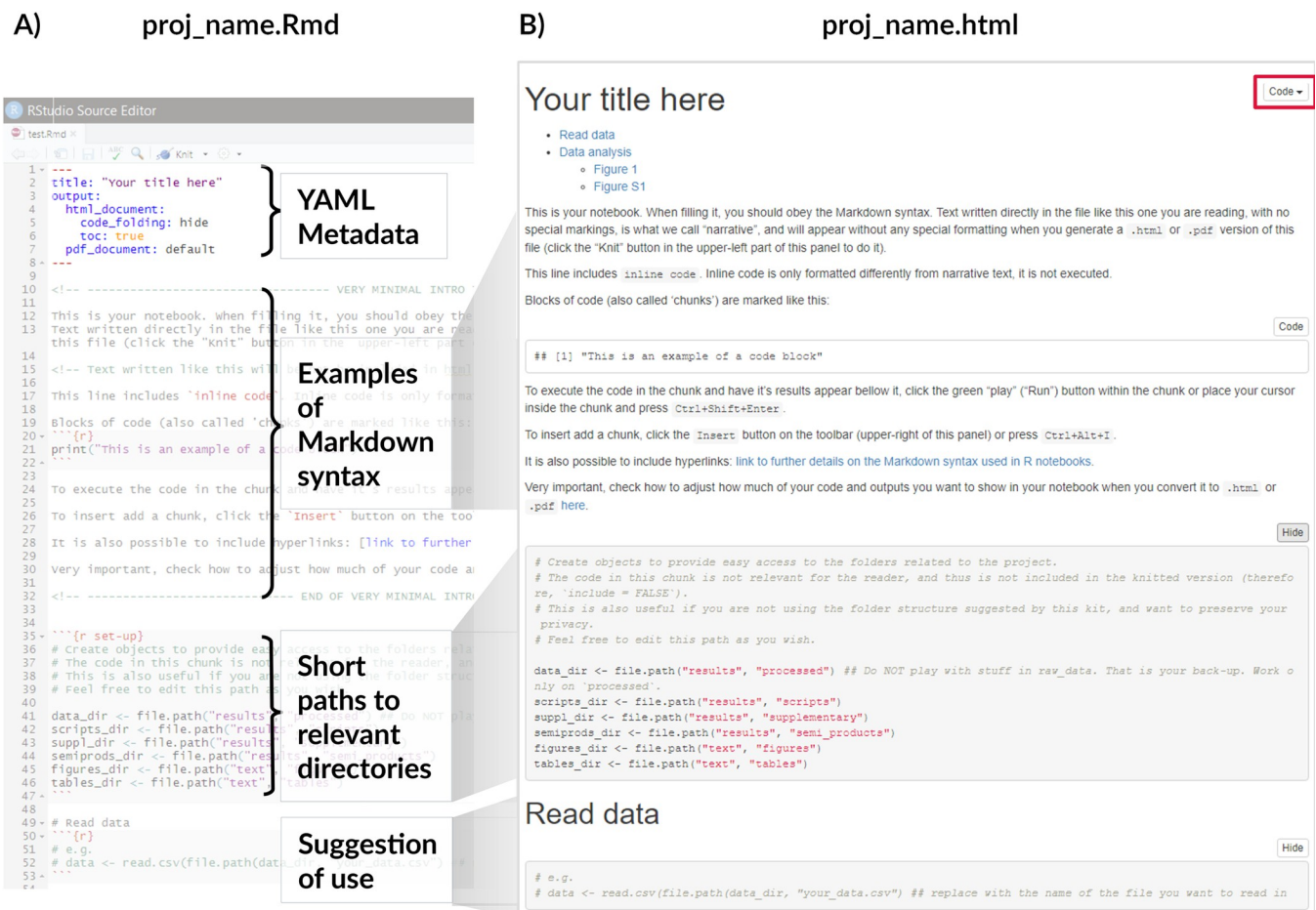
Fig 3. Comparison between the Rnotebook file available for editing (A) and the rendered html version (B). The function in set_kit.R creates an Rmd file (A) with basic metadata (title) and minimal formatting of the rendered file), a brief tutorial on the Markdown syntax, paths to the most relevant folders, and suggestions of use. In the html version (B), one can see how text and code are converted and combined, as well as a couple of features available in Rnotebooks: a table of contents, just below the title (defined by the toc argument set to true in the YAML section of the Rnotebook file), and a code button, that hides the blocks of code by default, to facilitate reading (defined by the code_folding argument set to hide in the YAML section). The video accompanying this tutorial details how the document works (available in https://github.com/FellowsFreiesWissen/computational_notebooks ).
