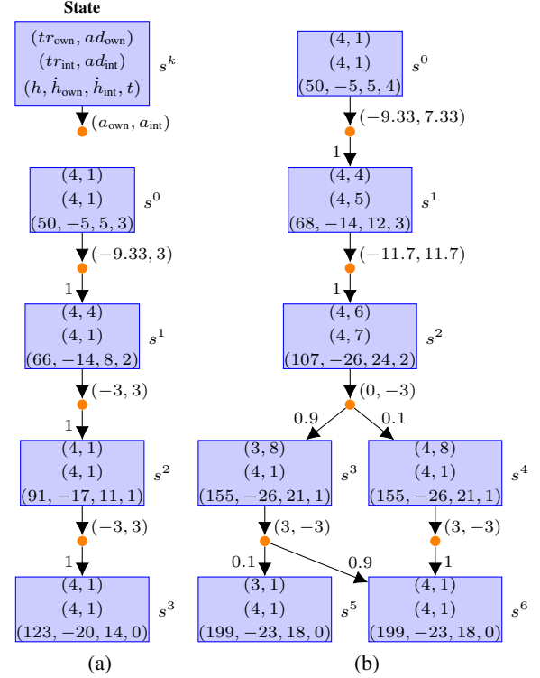
Figure 5: Strategies for the VCAS[2] example: (a) \epsilon_{own} = 0 , \epsilon_{int} = 0 and t initially 3; (b) \epsilon_{own} = 0.1 , \epsilon_{int} = 0 and t initially 4.
