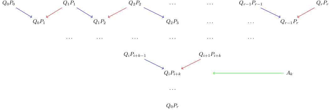
FIGURE 1. Lifted Darboux coordinates for the Takiff algebra of degree r . In this diagram we have r + 1 rows, and we number them starting at the top with row 0, all the way down to row r . The sum of the elements in row k gives the coefficient A_k of the power of z^{-k-1} , the blue arrow follows each Q_i matrix from the formula above to the one below, while the red one follows P_i .
