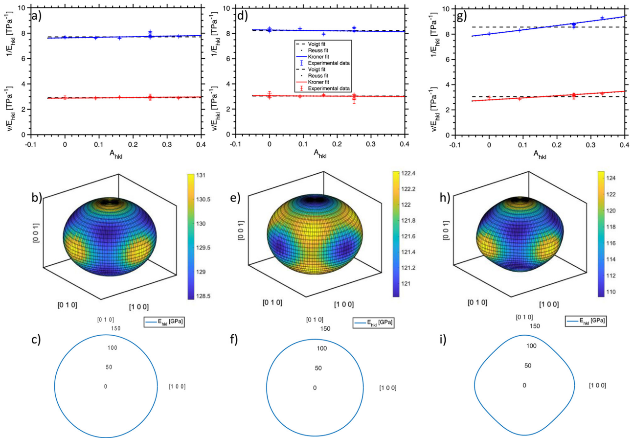
Fig. 6. Figures demonstrating the directional variation of V44's elastic properties: a), b), and c) at room temperature, d), e), and f) at 550°C, g), h), and i) at 700°C. Figs. a), d), and g) demonstrate the dependency of the plane specific elastic constants on elastic anisotropy including the fit provided by the Voigt, Reuss, and Kroner models used to determine the single crystal elastic constants. The legend provided in Fig. 6d) applies to a), d), and g). Figs. b), e) and h) show the three dimensional variation of elastic modulus with direction, and Figs. c), f) and i) are a projection of this modulus-direction dependency onto the XY plane.
