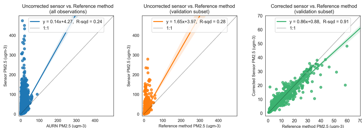
Figure 8. Relationship between uncorrected sensor, RF-model-corrected sensor and reference method observations for \text{PM}_{2.5} . The dotted line shows the unity slope. R-sqd: R^2 . \mu\text{g m}^{-3} .
