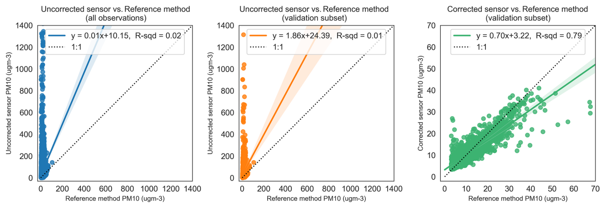
Figure 7. Relationship between uncorrected sensor, RF-model-corrected sensor and reference method observations for PM 10 . The dotted line shows the unity slope. R-sqd: R^2 . \mu\text{g m}^{-3} .
