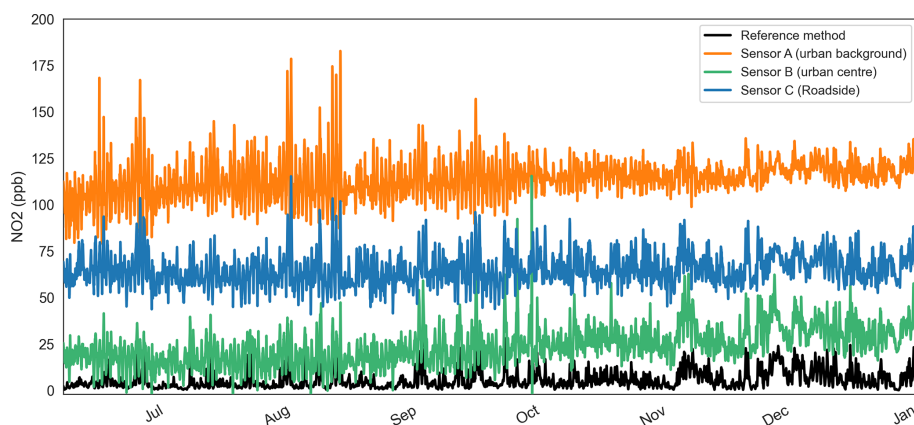
Figure 4. A 3 h rolling mean raw low-cost sensor and reference method NO 2 time series at three locations in Oxford for 2020.
