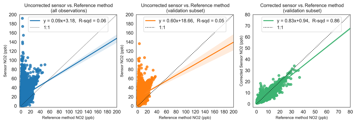
Figure 6. Relationship between uncorrected sensor, RF-model-corrected sensor and reference method observations for NO 2 . The dotted line shows the unity slope. R-sqd: R^2 .
