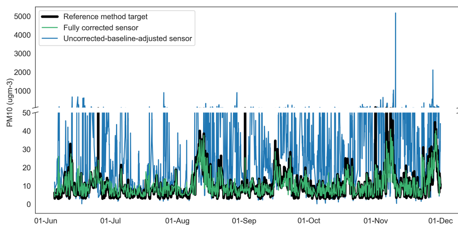
Figure 10. Time series of uncorrected-baseline-adjusted sensor, fully corrected sensor and reference method observations for PM 10 at Oxford St Ebbe's for 2020. ugm-3: \mu\text{g m}^{-3} .
