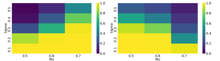
Fig. 4. Fraction of rejected cases for the AD (left) and tAD (right) tests on the Cut Cauchy scenario, based on its parameterizations. The used sample size is 100, with \alpha = 0.01 and no multiple comparison correction applied.
