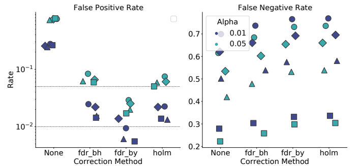
Fig. 9. Evaluation of multiple comparison correction methods: fraction of false positives in 30D samples with different correction methods (on the left) and aggregated fraction of False Negatives across all scenarios of the 6 most distinguishing tests based on Shapley values (on the right). On the left, values above the relevant \alpha -thresholds (0.01, 0.05) indicate too large false positive rates. On both figures, markers identify the used sample size: \circ , \diamond , \triangle and \square are 30, 50, 100 and 600, respectively. Here, we conclude that BY correction method should be chosen.
