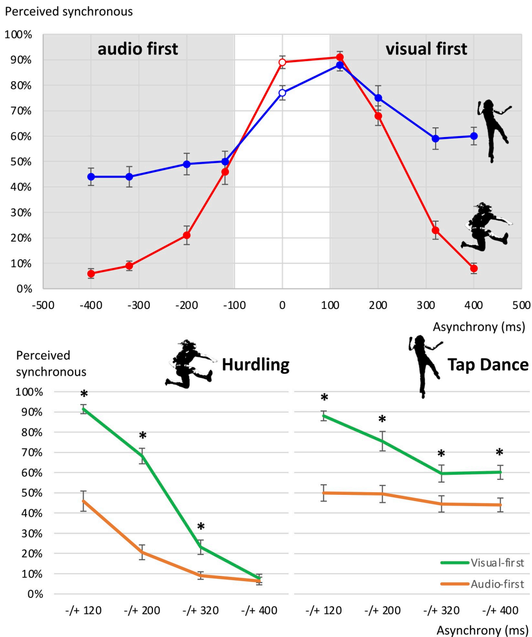
Fig 4. Mean percentages of trials perceived as synchronous, Study 1. Asynchronies (in ms) are displayed on the x-axis, with negative values indicating that the auditory channel preceded the visual channel (audio-first) and positive values indicating that the visual channel preceded the auditory channel (visual-first). Error bars show standard error of the mean. The upper panel shows all scores, fanned out for the level combinations of the factors asynchrony size, asynchrony type, and action type. The lower panel illustrates the significant action x asynchrony size x asynchrony type interaction.
