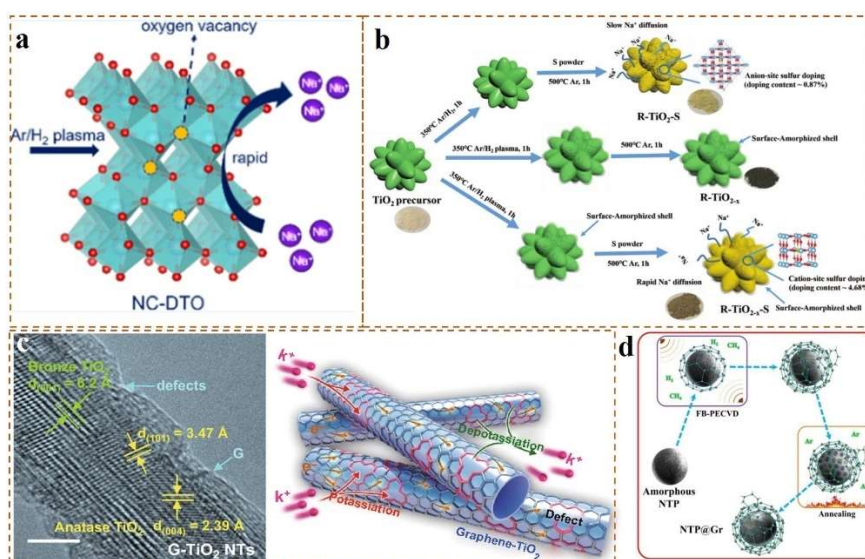
Figure 7. a) the schematic mechanism of NC-DTO. Reproduced with permission [120], Copyright 2018, American Chemical Society. b) the synthesis process for R-TiO 2 -S, R-TiO 2-x , and R-TiO 2-x -S. Reproduced with permission [127], Copyright 2018, Wiley-VCH. c) HRTEM image of as-prepared G-TiO 2 NTs, and the schematic
