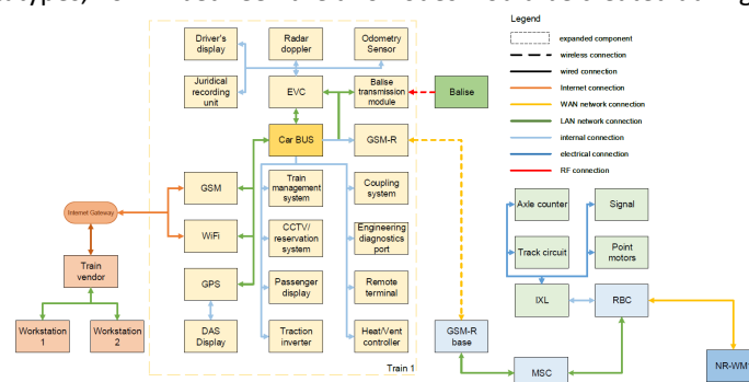
Figure 2: Model of ERTMS, with a train expanded into its constituent components.
