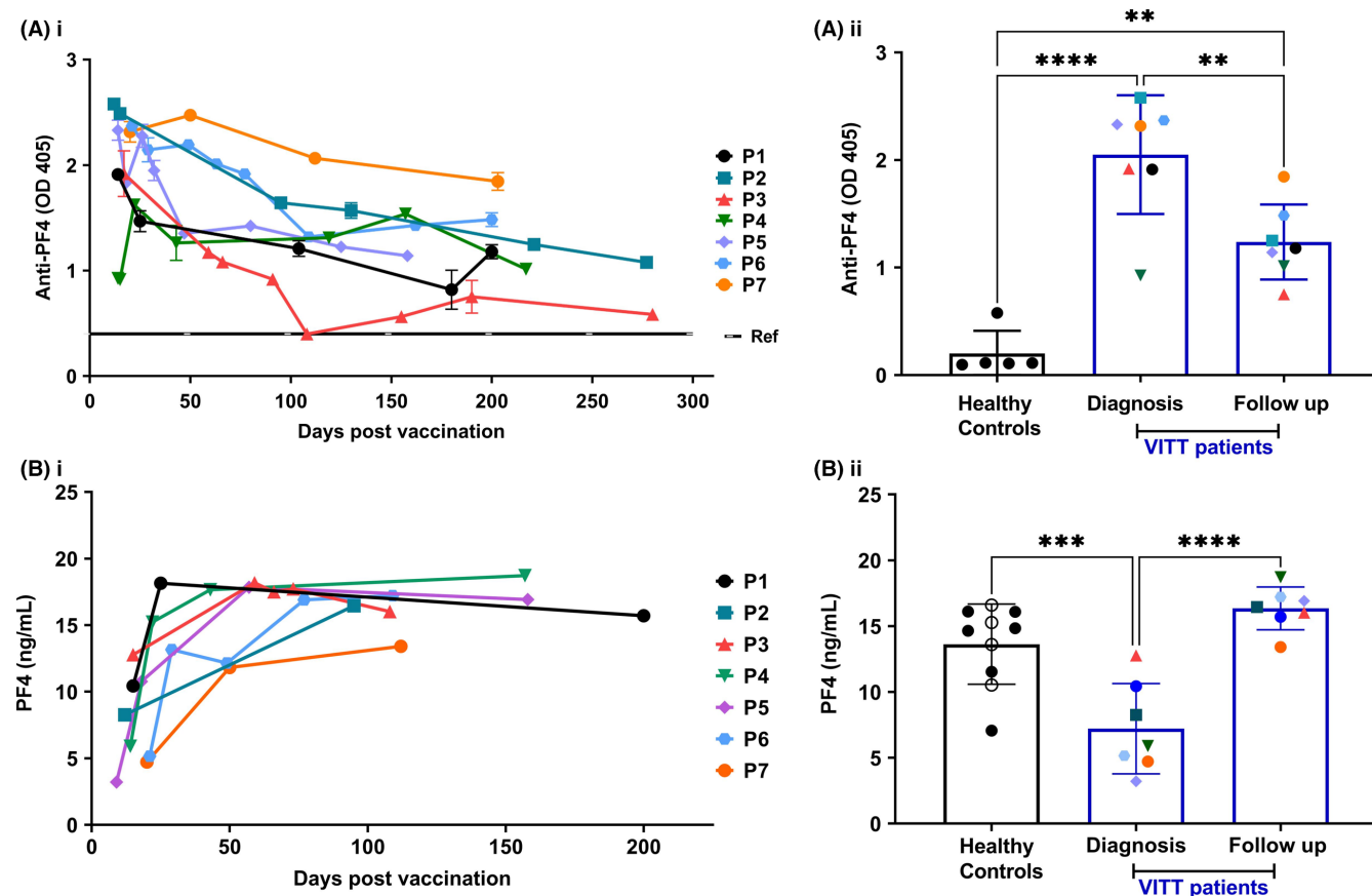
FIGURE 2 Levels of anti-PF4 IgG and PF4 level's in the serum of patients with VITT during follow-up. (Ai) Serum anti-PF4 levels of VITT patients ( n = 7 ) at diagnosis and during follow-up timepoints after vaccination. Samples measured in duplicate, mean \pm SEM. OD 405, optical density at 405 nm. Ref, clinical control reference range <0.4 O.D. (Aii) Patient serum anti-PF4 IgG levels at diagnosis and later follow-up timepoint (nearest to 200 days) ( n = 7 ) compared with healthy control serum levels ( n = 5 , including serum from the three responsive donors). Individual patient symbol corresponds to patient labels in (i). Results reported as mean \pm SD. One-way ANOVA with Tukey's multiple comparison test, **p < 0.01 , ****p < 0.0001 . (Bi) Serum PF4 levels of all patients with VITT ( n = 7 ) at diagnosis and follow-up timepoints after vaccination. (Bii) Patient serum PF4 levels at diagnosis and latest follow-up timepoint ( n = 7 ) compared with healthy controls ( n = 10 ), including AZD1222-vaccinated individuals ( n = 4 , open circle). Individual patient symbol corresponds to patient labels in (i). Results reported as mean \pm SD. One-way ANOVA with Tukey multiple comparison test, ***p = 0.0005 , ****p < 0.0001
