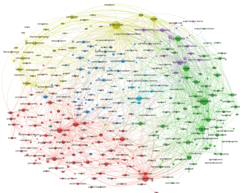
Figure 3. Co-occurrence network of terms, colour-coded by cluster.
