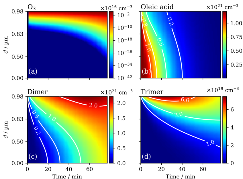
Figure 4. Spatially and temporally resolved concentration evolution of ozone ( a – log-scale concentration), oleic acid ( b ), dimer ( c ) and trimer ( d ) model components during ozonolysis for a 0.98 \mu\text{m} film – d : the distance from the film–substrate interface. Contours illustrate the change in concentration gradient over time for the non-reactive gas species. [\text{O}_3] = 77 ppm.
