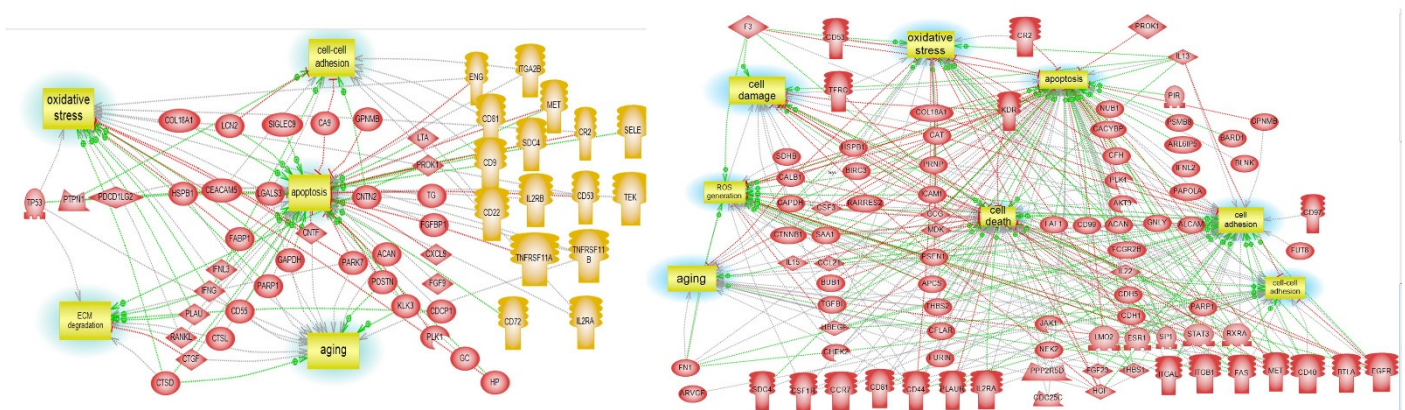
Figure 6. DE-protein pathway studio analyses in Braak III-IV and Braak V-VI. AD pathways generated by DE-proteins in Braak III-IV (panel A) and Braak V-VI DE-miRNA (panel B).
