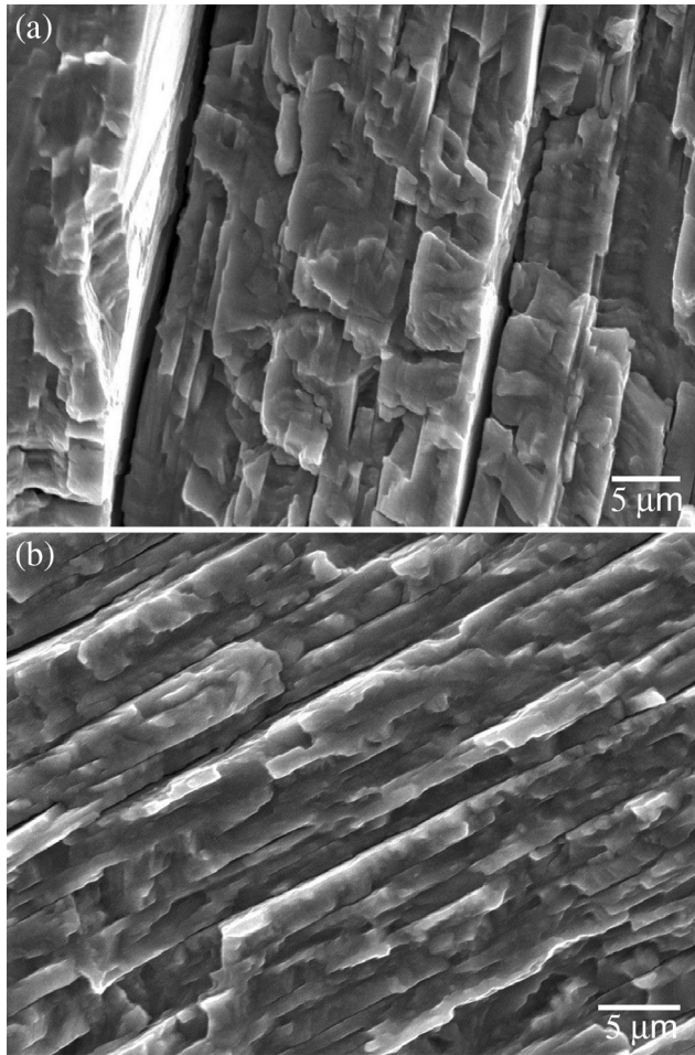
Fig. 6. Translamellar fracture at high \Delta K ; (a) 15.5 and (b) 16.2 MPa/m.
