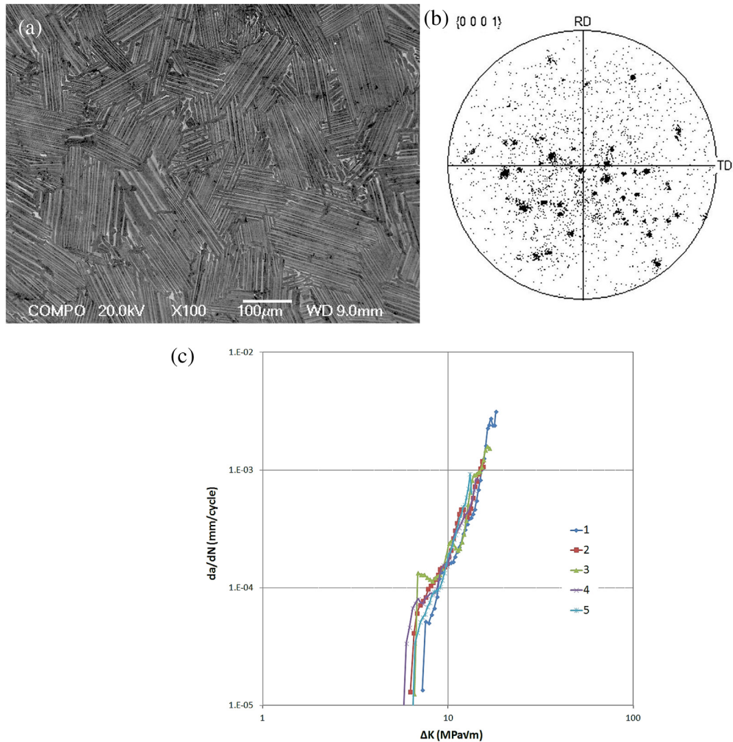
Fig. 1. (a) SEM BSE image showing the lamellar microstructure of investment cast Ti45Al2Mn2Nb1B and (b) the EBSD (0001)_{\alpha_2} pole figure shows the random lamellar orientation distribution. (c) Fatigue crack propagation curves at 650 °C with R = 0.1 .
