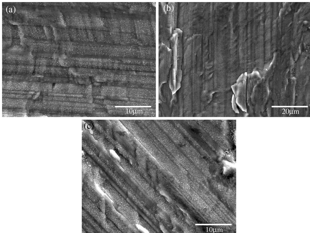
Fig. 5. Translamellar fracture at low \Delta K ; (a) 7.5, (b) 6.4, and (c) 6.5 \text{MPa}\sqrt{\text{m}} .
