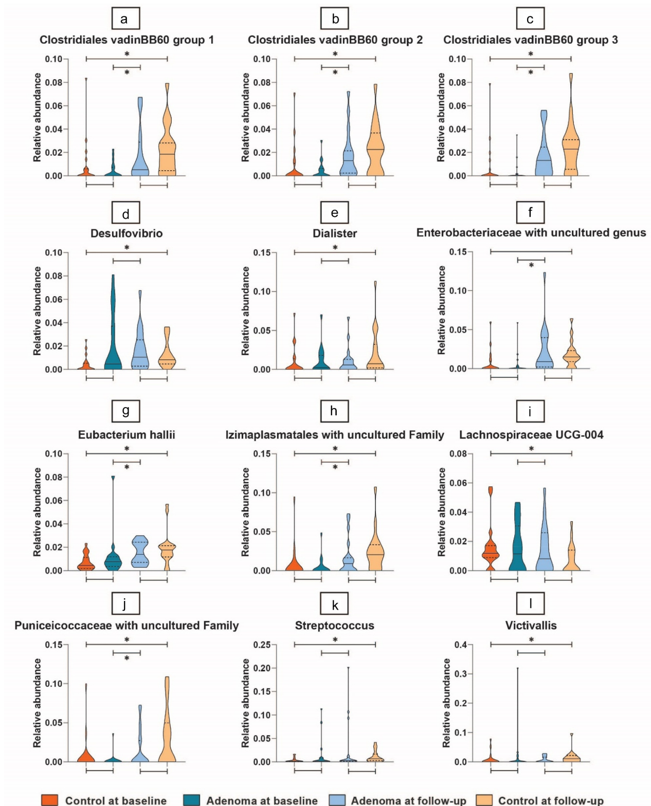
Figure 3. Distribution of selected taxa for baseline versus follow-up. The distribution of taxa selected to differentiate between baseline and follow-up across all four subgroups. Depicted are the microbial taxa meeting the criteria of significance of a Linear Discriminant Analysis (LDA) value >2 . On the Y-axis, the relative abundance per taxa is presented in violin plots. On the X-axis, study groups are given. Dark Orange depicts control samples at baseline, dark blue depicts adenomas at baseline, light blue depicts adenomas at follow-up, light-orange depicts controls at follow-up. The horizontal line within the violin plots represents the median and the dotted lines represent the upper and lower quartiles. Broadness of the violin plot depicts the density of samples at the corresponding taxa relative abundance. Significance is indicated by a star above of under the lines connecting study groups.
