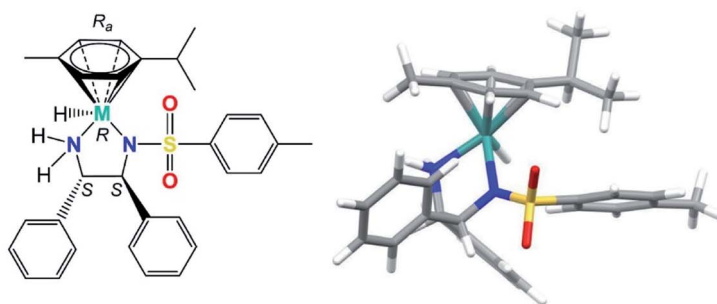
Fig. 3 Structures of the R -configured hydride complex [M( p -cymene)( S,S -TsDPEN-H)H], where M = Ru or Os showing the axial chirality involving rotation of the \pi -bonded p -cymene ligand: (a) S a axial chirality (0 kJ mol -1 ) and (b) R a axial chirality (5 kJ mol -1 ). Note that the chelated ligand contains a protonated NH group (as NH 2 in TsDPEN-H), which facilitates hydride transfer to the metal (Fig. S4 and S5, PDB1 and PDB2). †
