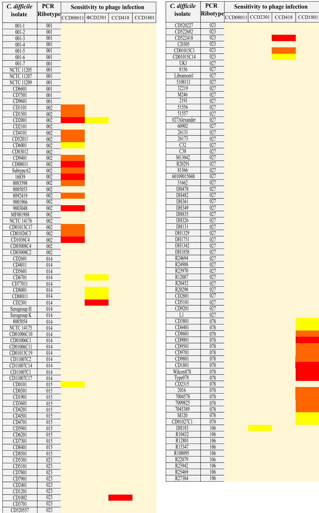
FIG 3 Heat map of C. difficile sensitivity to bacteriophage infection. Phage host range was determined using standard plaque assays for phages ΦCD08011, ΦCD2301, ΦCD418, and ΦCD1801. Efficiency of plating (EOP) values are depicted for each infection study represented by color. Magnolia, resistant strain; yellow, EOP of <0.1; orange, EOP 0.1 to 1; red, EOP of >1.
