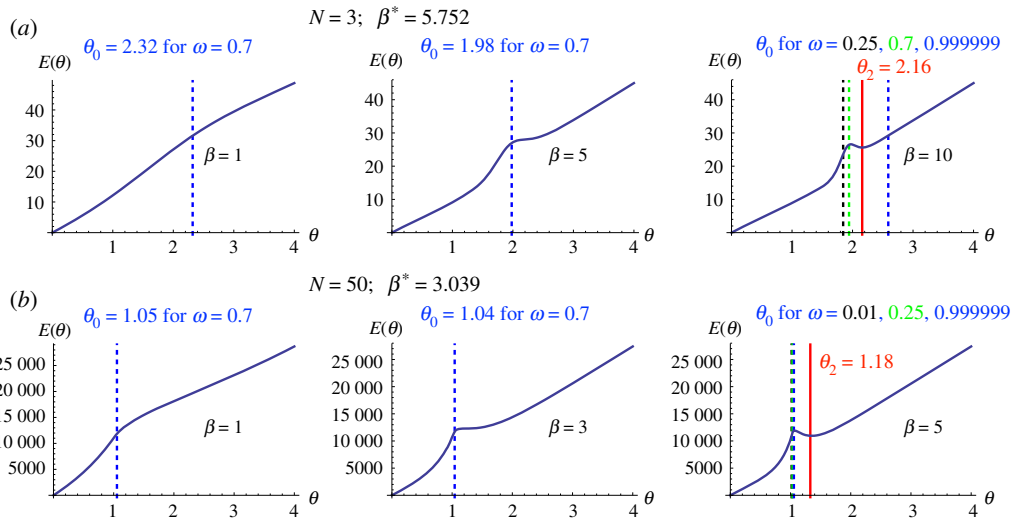
Figure 3. We use algorithm 3.3 to find optimal \theta that minimizes E(\theta) (for institutional reward) while ensuring a minimum level of cooperation \omega . We also use as examples a small population size ( N = 3(a) ) and a larger one ( N = 50(b) ), for DG ( b = 1.8 , c = 1 ). (Online version in colour.)
