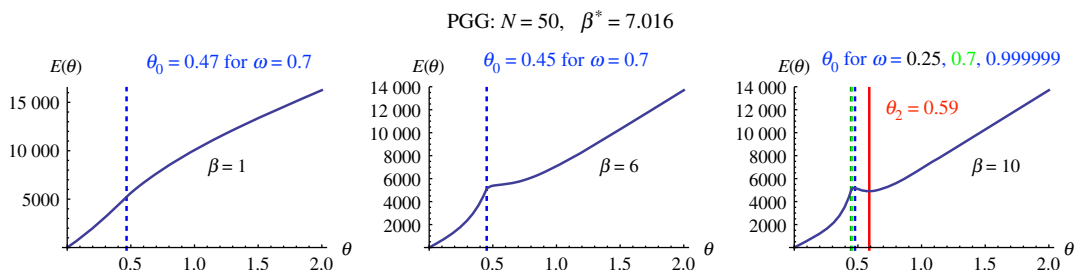
Figure 4. We use algorithm 3.3 to find optimal \theta that minimizes E(\theta) while ensuring a minimum level of cooperation \omega , for PGG ( r = 3 , n = 5 , c = 1 ) with N = 50 . Similar observations to those for DG are obtained. (Online version in colour.)
