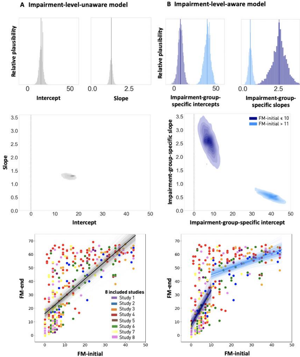
Figure 4. Motor stroke outcome is best explained by initial-impairment-dependent recovery patterns. A. Impairment-level-unaware model. The interpretation of intercepts and slopes of this model led to the conclusion of a combination of constant and proportional to spared recovery for the entirety of patients. However, this model was consistently outperformed by all impairment-level-aware models, indicating the benefit of assuming two subgroups within the entire patient cohort. B. Impairment-level-aware model employing a breakpoint of FM\text{-}initial=10 to differentiate between severely and non-severely affected patients. We here observed two distinct recovery patterns:
