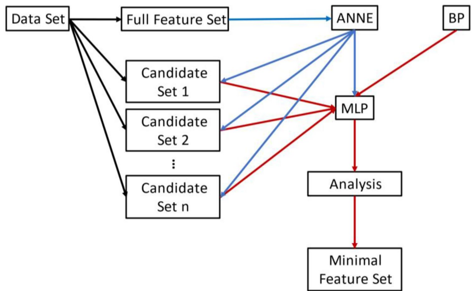
Fig. 3 Steps of feature relevance analysis split into two stages. In the first stage (blue lines), the ANNE procedure was used to optimise the MLP structure and generate candidate groups of surface parameters. In the second stage (red lines), the parameter groups were evaluated on the learning results of MLP (using BP training) and a final minimal group of relevant areal surface parameters is generated
