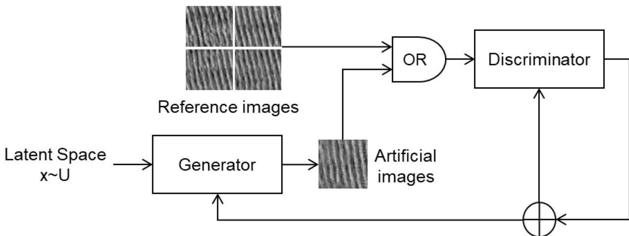
Fig. 2 Schematic representation of GAN used to generate artificial height maps/depth images based on experimental LIPSS topography data. The loss signal of the Generator is the opposite of the loss sig-
