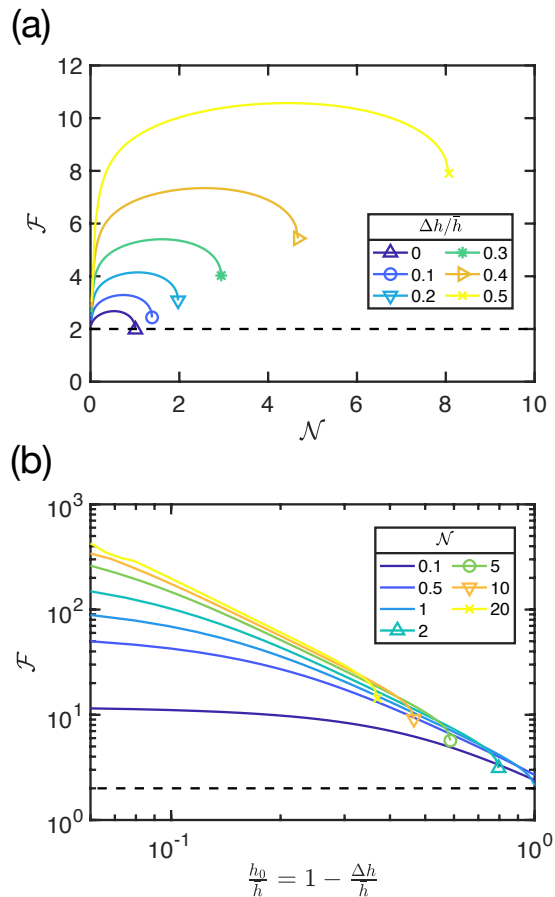
Figure 6: The dimensionless total adhesion force as a function of (a) the scaled number of bridges, \mathcal{N} = n/(V_{\text{tot}}/\bar{h}^3) , at fixed roughness amplitudes \Delta h/\bar{h} = \{0, 0.1, 0.2, 0.3, 0.4, 0.5\} (plotted up to rupture, which is indicated by symbols), and (b) the minimum gap width, h_0/\bar{h} = 1 - \Delta h/\bar{h} , with fixed number of bridges \mathcal{N} = \{0.1, 0.5, 1, 2, 5, 10, 20\} . In both cases here \theta = 0 and \alpha = 10 , and results are compared to a dashed line denoting eqn. (2). Note that in (a), the case \Delta h = 0 corresponds to the case of flat plates studied by De Souza et al. [37].
