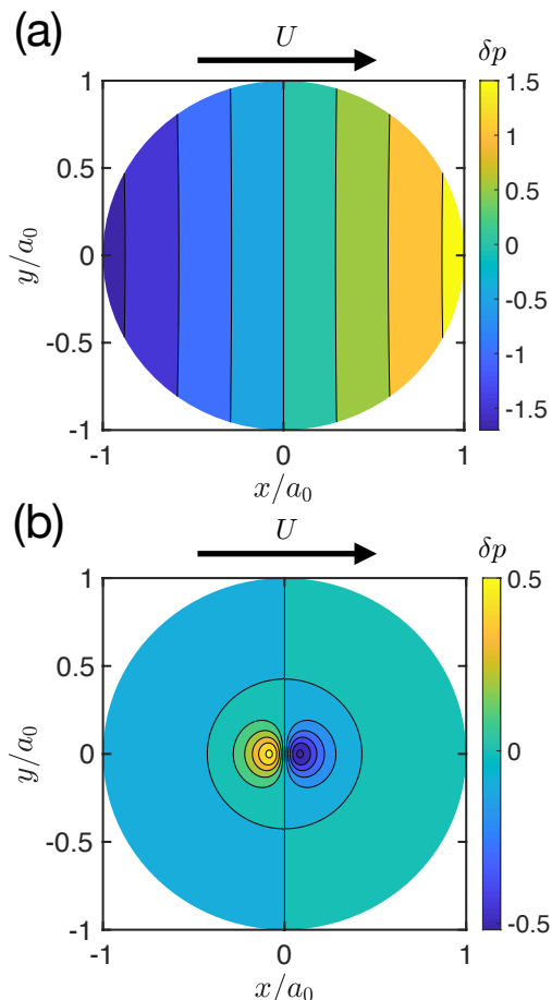
Figure 8: The first order correction to the (dimensionless) pressure field inside the bridge, \delta p(x, y) = (p - p_0)/(Ca \gamma \cos \theta / h_0) as it is sheared in steady state for (a) V/(Rh_0^2) = 1 and (b) V/(Rh_0^2) = 100 . The leading order pressure is uniform, p_0 = -2\bar{\gamma}/h(a_0) . Note that the radial lengths have been rescaled so that the equilibrium position has r = 1 in these images; the corresponding equilibrium radii are a_0/\sqrt{Rh_0} = 0.30 and 9.5 , respectively. The deviation in meniscus position is not illustrated for simplicity.
