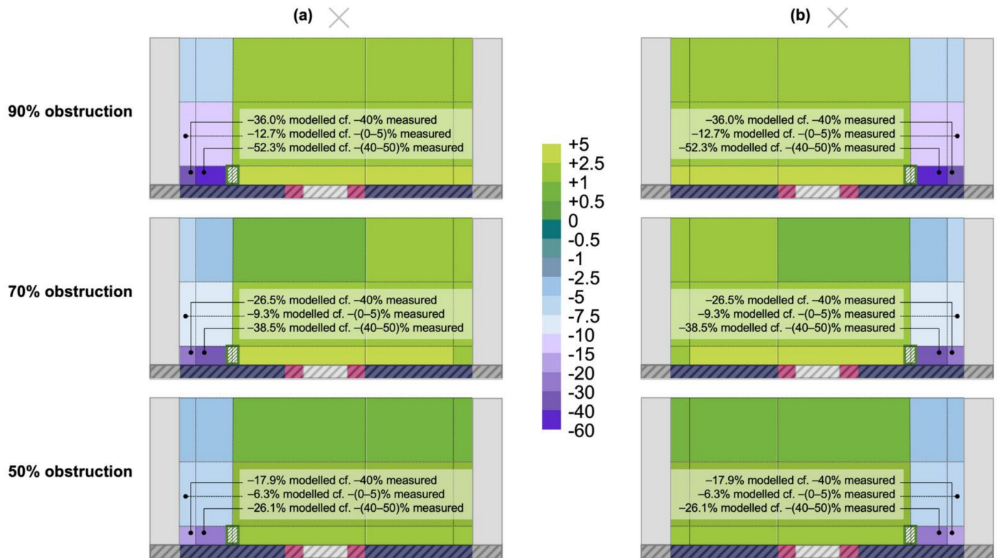
Figure 11. Modelled changes in SF 6 mass concentration (%), on introducing a roadside barrier in a street canyon under parallel wind conditions aloft, when the barrier is located (a) on the left of the street, and (b) on the right of the street, as we seek to emulate [49]’s wind tunnel measurements.
