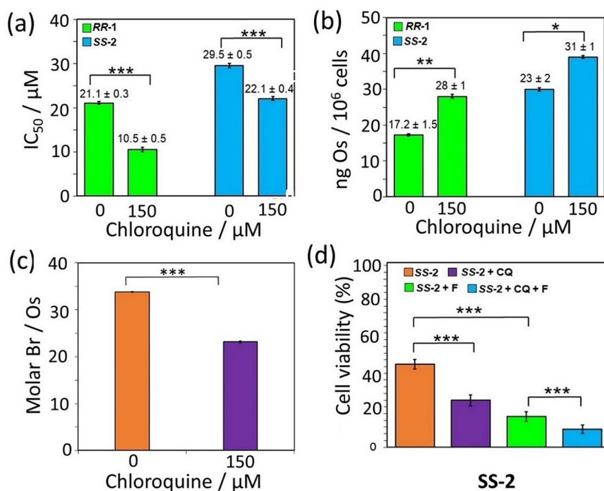
Figure 5. a) Half-maximal inhibitory concentrations ( IC_{50} /μM) of R,R -1 and S,S -2 for A549 (human lung) cancer cells pre-incubated with 0 or 150 μM of chloroquine diphosphate for 2 h, followed by 24 h complex exposure and 72 h recovery period in fresh media. b) Accumulation of Os ( ^{189}Os ; ng/ 10^6 cells) in A549 cells pre-incubated with 0 or 150 μM chloroquine diphosphate for 2 h and treated with 1 \times IC_{50} of R,R -1 (21 μM) or S,S -2 (30 μM) for 24 h. c) Molar Br-to-Os ratios (Br/Os) for A549 cells pre-incubated with 0 or 150 μM of chloroquine diphosphate for 2 h and treated with 1 \times IC_{50} of S,S -2 (30 μM) for 24 h. d) Transfer hydrogenation-modulated cellular viability of human A549 cells pre-incubated with 0 or 150 μM chloroquine diphosphate for 2 h and treated with 1 \times IC_{50} of S,S -2 in the presence of formate (0–2 mM). Statistical significance was calculated using a two-tailed t-test assuming unequal variances (Welch's t-test), * p < 0.05 , ** p < 0.01 and *** p < 0.001 .
