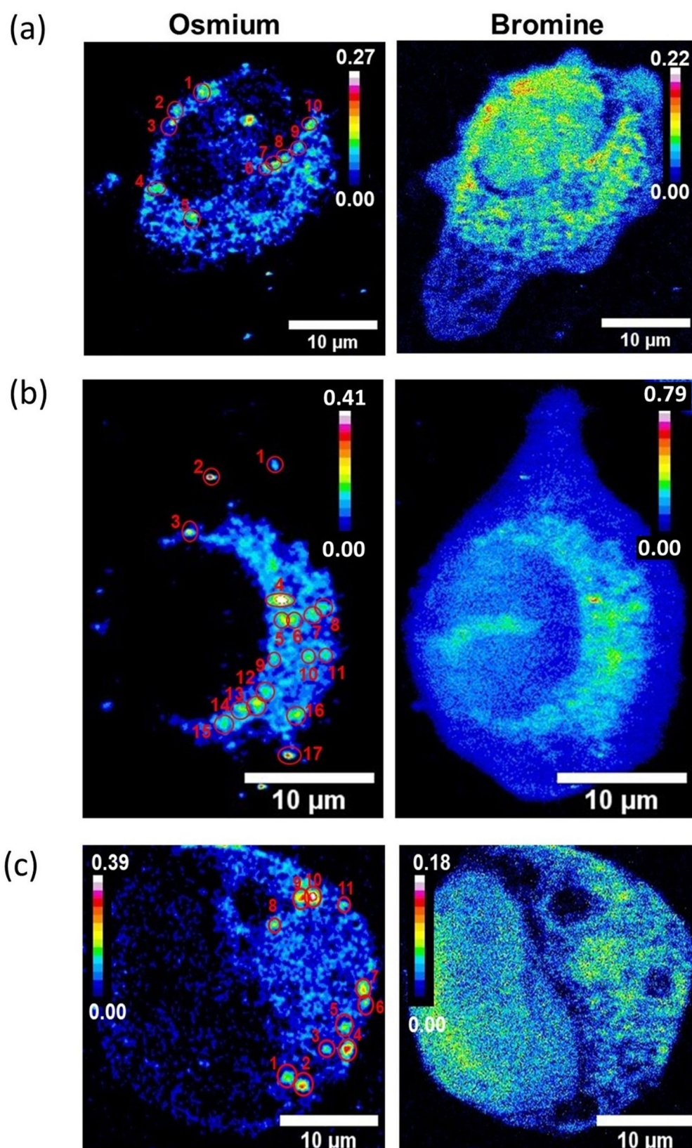
Figure 4. XRF elemental maps of Os and Br acquired from cryo-fixed and freeze-dried A549 (human lung) cancer cells treated with a) 1, b) 3 or c) 5 \times \text{IC}_{50} of S,S -2 (30, 90 or 150 μM) for 24 h, showing Os-Br co-localisation in small vesicle-like areas. Maps were collected using 100 nm step size and 0.1 s dwell time. The calibration bar is in \text{pg mm}^{-2} . Data were processed using the PyMCA toolkit developed by the ESRF, [15] and images generated in ImageJ. [16]
