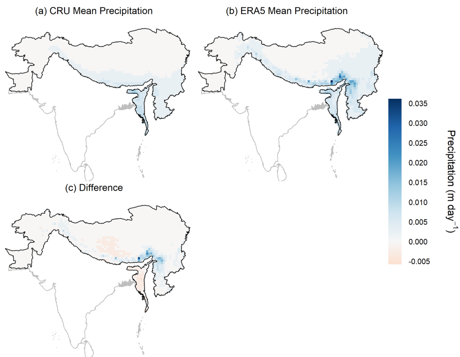
Figure 10. Comparison of precipitation (a) average CRU (1960–1990), (b) ERA5 data (1979–1990) and (c) the difference between the ERA5 and CRU datasets in m d -1 .
