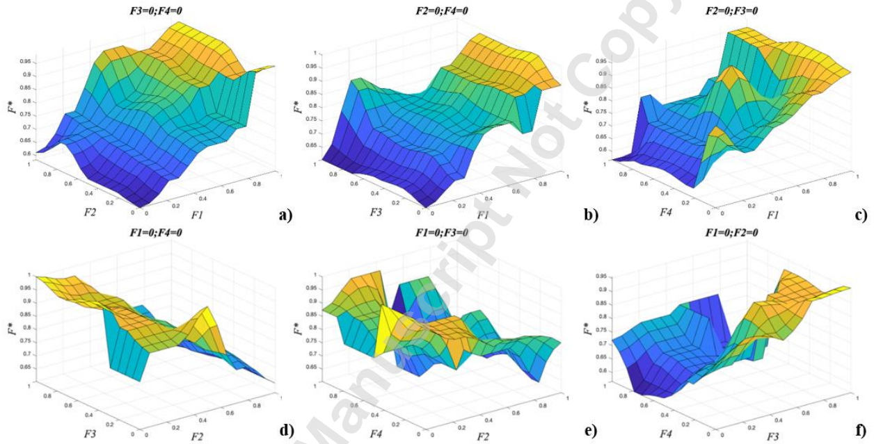
Fig. 6. Inputs/output mapping of the ANFIS: a) F1 and F2 to F*; b) F1 and F3 to F*; c) F1 and F4 to F*; d) F2 and F3 to F*; e) F2 and F4 to F*; f) F3 and F4 to F*
