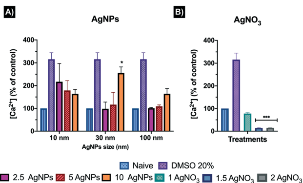
Fig. 5 Intracellular calcium induced by (A) AgNPs and (B) \text{AgNO}_3 in ZF4 cells at 24 hours in CCM. Cells were treated with 2.5, 5 and 10 \mu\text{g mL}^{-1} of 10, 30 and 100 \text{ nm} AgNP and 1, 1.5 and 2 \mu\text{g mL}^{-1} of \text{AgNO}_3 as ionic control for 24 hours. A positive control of 20\% DMSO was also included for 30 minutes to ensure the reliability of the assay. The obtained intensities were corrected by subtracting the mean of the naïve cells from all treatments, then the corrected intensities were normalized to an equal number of 1000 cells per treatment and finally transformed to percentage (%) against naïve. Results represent the mean and standard deviation of three individual replicates. Data with asterisks (*) indicate a statistically significant difference of AgNPs treatments (* p < 0.05 , and *** p < 0.001 ) compared to the naïve cells.
